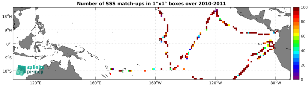
Figure 4: Number of SSS match-ups between TSG (GOSUD-Sailing-ship) SSS and the SMOS SSS L2Q v331 - No FLAG (CMEMS-CATDS-CPDC) SSS product for the Tropical Pacific Ocean Pi-MEP region over 1^\circ \times 1^\circ boxes and for the full satellite product period.
