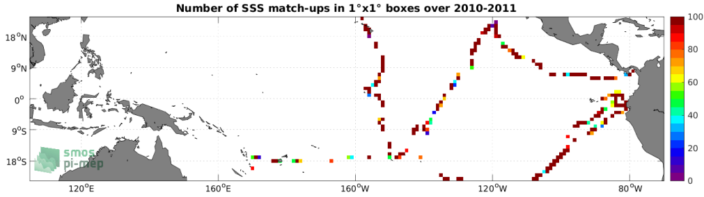
Figure 4: Number of SSS match-ups between TSG (GOSUD-Sailing-ship) SSS and the SMOS SSS L2Q v331 - No FLAG (CMEMS-CATDS-CPDC) SSS product for the Tropical Pacific Ocean Pi-MEP region over 1^\circ \times 1^\circ boxes and for the full satellite product period.
