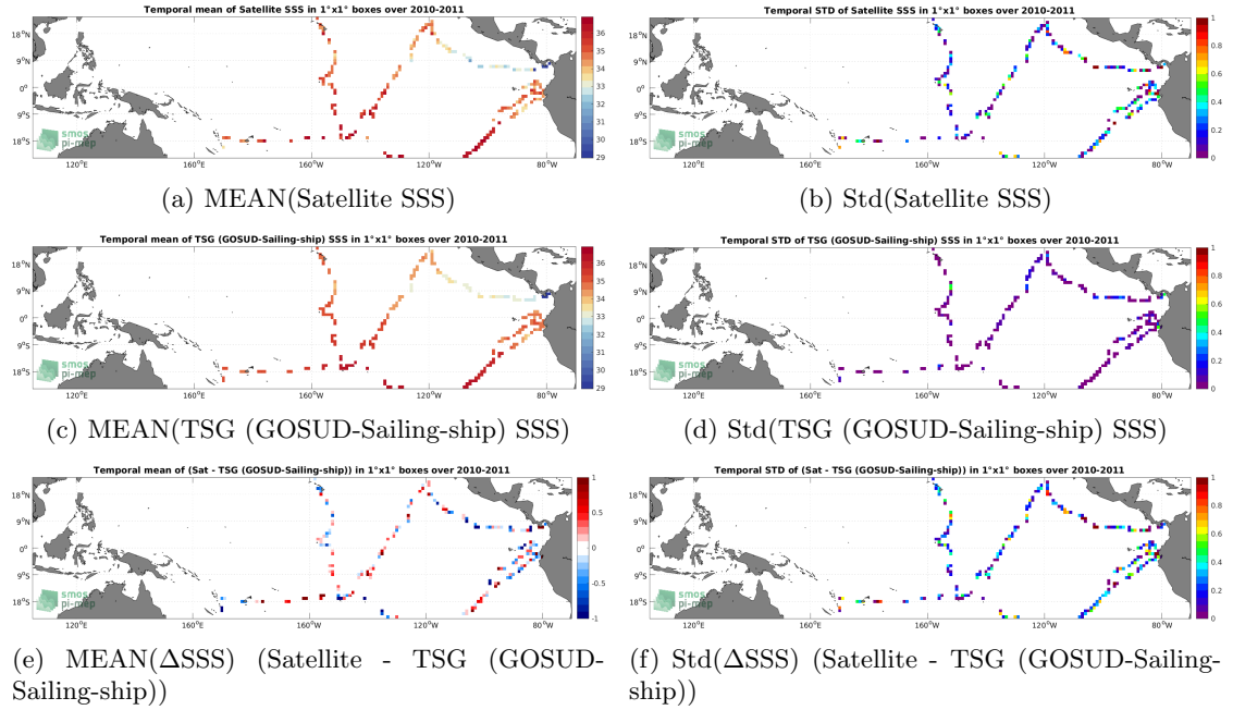
Figure 6: Temporal mean (left) and Std (right) of SSS from SMOS SSS L2Q v331 - No FLAG (CMEMS-CATDS-CPDC) (top), TSG (GOSUD-Sailing-ship) (middle), and of \Delta SSS (Satellite - TSG (GOSUD-Sailing-ship)). Only match-up pairs are used to generate these maps.
