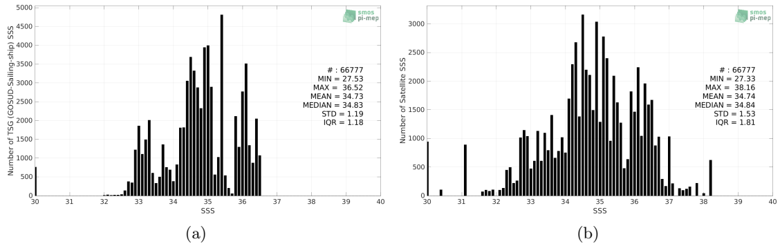
Figure 2: Histograms of SSS from TSG (GOSUD-Sailing-ship) (a) and SMOS SSS L2Q v331 - No FLAG (CMEMS-CATDS-CPDC) (b) considering all match-up pairs per bins of 0.1 over the Tropical Pacific Ocean Pi-MEP region and for the full satellite product period.
