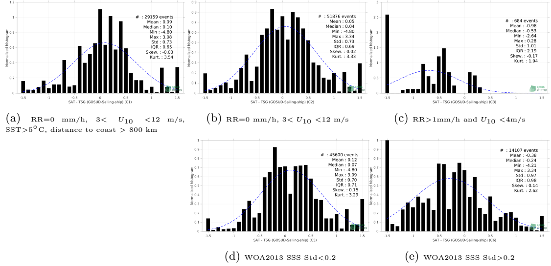
Figure 13: Normalized histogram of \Delta SSS (SMOS SSS L2Q v331 - No FLAG (CMEMS-CATDS-CPDC) - TSG (GOSUD-Sailing-ship)) for 5 different subdatasets corresponding to: RR=0 mm/h, 3 < U_{10} < 12 m/s, SST > 5°C, distance to coast > 800 km (a), RR=0 mm/h, 3 < U_{10} < 12 m/s (b), RR > 1mm/h and U_{10} < 4 m/s (c), WOA2013 SSS Std < 0.2 (d), WOA2013 SSS Std > 0.2 (e).
