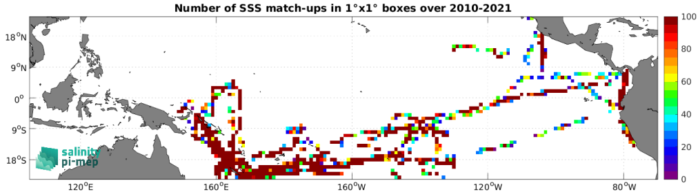
Figure 5: Number of SSS match-ups between TSG (GOSUD-Research-vessel) SSS and the SMOS SSS L2Q v331 - No FLAG (CMEMS-CATDS-CPDC) SSS product for the Tropical Pacific Ocean Pi-MEP region over 1^\circ \times 1^\circ boxes and for the full satellite product period.
