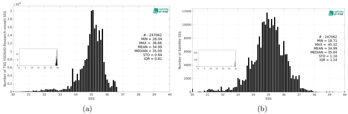
Figure 3: Histograms of SSS from TSG (GOSUD-Research-vessel) (a) and SMOS SSS L2Q v331 - No FLAG (CMEMS-CATDS-CPDC) (b) considering all match-up pairs per bins of 0.1 over the Tropical Pacific Ocean Pi-MEP region and for the full satellite product period.
