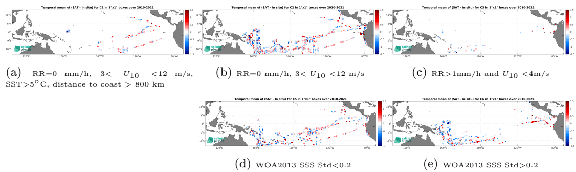
Figure 12: Temporal mean gridded over spatial boxes of size 1^\circ \times 1^\circ of \Delta SSS (SMOS SSS L2Q v331 - No FLAG (CMEMS-CATDS-CPDC) - TSG (GOSUD-Research-vessel)) for 5 different subdatasets corresponding to:RR=0 mm/h, 3 < U_{10} < 12 m/s, SST > 5^\circ\text{C} , distance to coast > 800 km (a), RR=0 mm/h, 3 < U_{10} < 12 m/s (b), RR > 1 mm/h and U_{10} < 4 m/s (c), WOA2013 SSS Std < 0.2 (d), WOA2013 SSS Std > 0.2 (e).
