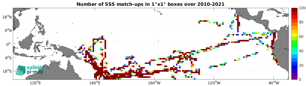
Figure 4: Number of SSS match-ups between TSG (GOSUD-Research-vessel) SSS and the SMOS SSS L2Q v331 - No FLAG (CMEMS-CATDS-CPDC) SSS product for the Tropical Pacific Ocean Pi-MEP region over 1^\circ \times 1^\circ boxes and for the full satellite product period.
