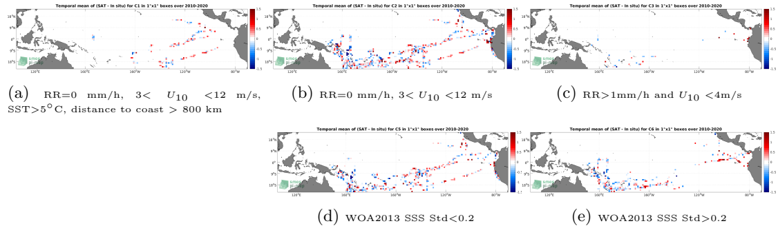
Figure 12: Temporal mean gridded over spatial boxes of size 1^{\circ}\times 1^{\circ} of \Delta SSS (SMOS SSS L2Q v331 - No FLAG (CMEMS-CATDS-CPDC) - TSG (GOSUD-Research-vessel)) for 5 different subdatasets corresponding to:RR=0 mm/h, 3 < U_{10} < 12 m/s, SST >5^{\circ}\text{C} , distance to coast > 800 km (a), RR=0 mm/h, 3 < U_{10} < 12 m/s (b), RR >1 mm/h and U_{10} < 4 m/s (c), WOA2013 SSS Std <0.2 (d), WOA2013 SSS Std >0.2 (e).
