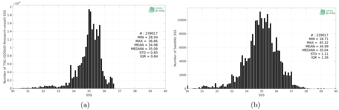
Figure 2: Histograms of SSS from TSG (GOSUD-Research-vessel) (a) and SMOS SSS L2Q v331 - No FLAG (CMEMS-CATDS-CPDC) (b) considering all match-up pairs per bins of 0.1 over the Tropical Pacific Ocean Pi-MEP region and for the full satellite product period.
