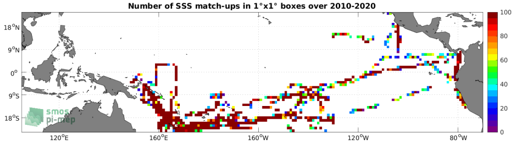
Figure 4: Number of SSS match-ups between TSG (GOSUD-Research-vessel) SSS and the SMOS SSS L2Q v331 - No FLAG (CMEMS-CATDS-CPDC) SSS product for the Tropical Pacific Ocean Pi-MEP region over 1^\circ \times 1^\circ boxes and for the full satellite product period.
