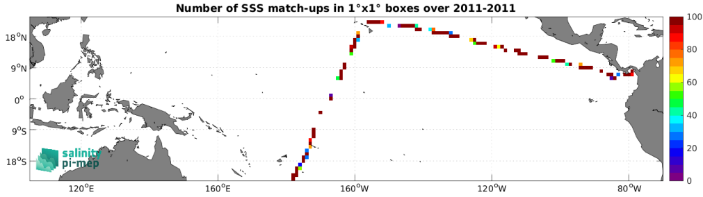
Figure 5: Number of SSS match-ups between TSG (CSIC-UTM) SSS and the SMOS SSS L2Q v331 - No FLAG (CMEMS-CATDS-CPDC) SSS product for the Tropical Pacific Ocean Pi-MEP region over 1^\circ \times 1^\circ boxes and for the full satellite product period.
