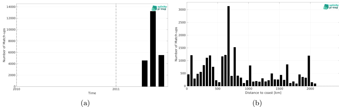
Figure 2: Number of match-ups between TSG (CSIC-UTM) and SMOS SSS L2Q v331 - No FLAG (CMEMS-CATDS-CPDC) SSS as a function of time (a) and as function of the distance to coast (b) over the Tropical Pacific Ocean Pi-MEP region and for the full satellite product period.
