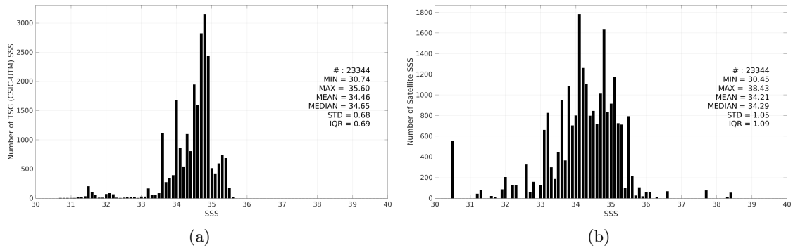
Figure 3: Histograms of SSS from TSG (CSIC-UTM) (a) and SMOS SSS L2Q v331 - No FLAG (CMEMS-CATDS-CPDC) (b) considering all match-up pairs per bins of 0.1 over the Tropical Pacific Ocean Pi-MEP region and for the full satellite product period.
