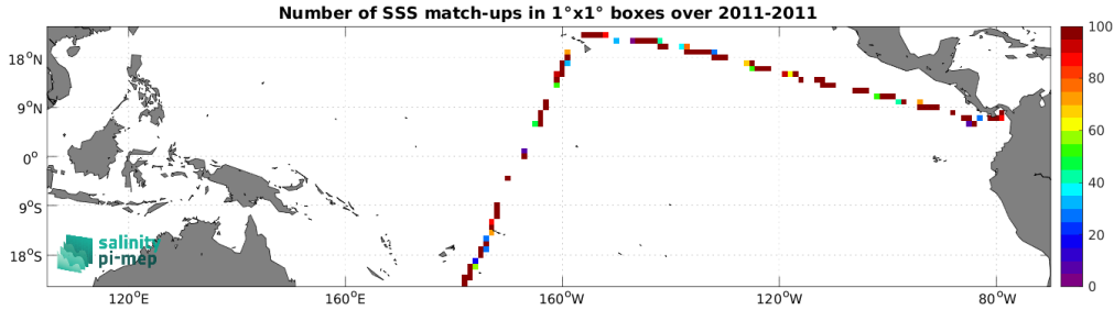
Figure 4: Number of SSS match-ups between TSG (CSIC-UTM) SSS and the SMOS SSS L2Q v331 - No FLAG (CMEMS-CATDS-CPDC) SSS product for the Tropical Pacific Ocean Pi-MEP region over 1^\circ \times 1^\circ boxes and for the full satellite product period.
