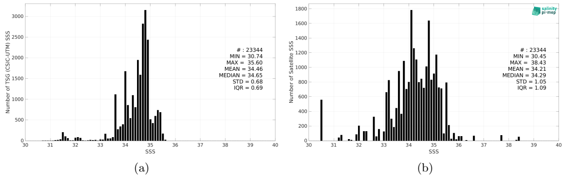
Figure 2: Histograms of SSS from TSG (CSIC-UTM) (a) and SMOS SSS L2Q v331 - No FLAG (CMEMS-CATDS-CPDC) (b) considering all match-up pairs per bins of 0.1 over the Tropical Pacific Ocean Pi-MEP region and for the full satellite product period.
