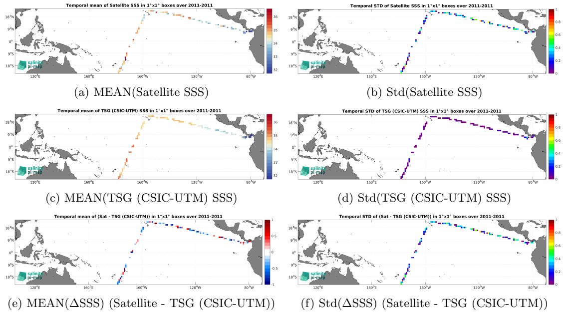
Figure 6: Temporal mean (left) and Std (right) of SSS from SMOS SSS L2Q v331 - No FLAG (CMEMS-CATDS-CPDC) (top), TSG (CSIC-UTM) (middle), and of \Delta SSS (Satellite - TSG (CSIC-UTM)). Only match-up pairs are used to generate these maps.
