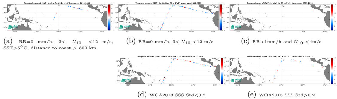
Figure 12: Temporal mean gridded over spatial boxes of size 1^{\circ}\times 1^{\circ} of \Delta\text{SSS} (SMOS SSS L2Q v331 - No FLAG (CMEMS-CATDS-CPDC) - TSG (CSIC-UTM)) for 5 different subdatasets corresponding to:RR=0 mm/h, 3 < U_{10} < 12 m/s, SST >5^{\circ}\text{C} , distance to coast > 800 km (a), RR=0 mm/h, 3 < U_{10} < 12 m/s (b), RR >1 mm/h and U_{10} < 4 m/s (c), WOA2013 SSS Std <0.2 (d), WOA2013 SSS Std >0.2 (e).
