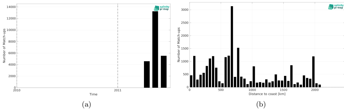
Figure 1: Number of match-ups between TSG (CSIC-UTM) and SMOS SSS L2Q v331 - No FLAG (CMEMS-CATDS-CPDC) SSS as a function of time (a) and as function of the distance to coast (b) over the Tropical Pacific Ocean Pi-MEP region and for the full satellite product period.
