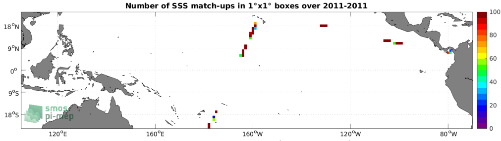
Figure 4: Number of SSS match-ups between TSG (CSIC-UTM) SSS and the SMOS SSS L2Q v331 - No FLAG (CMEMS-CATDS-CPDC) SSS product for the Tropical Pacific Ocean Pi-MEP region over 1^\circ \times 1^\circ boxes and for the full satellite product period.
