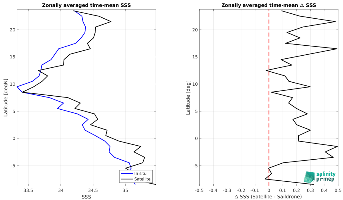
Figure 9: Left panel: Zonal mean SSS from SMOS SSS L2Q v331 - No FLAG (CMEMS-CATDS-CPDC) satellite product (black) and from Saildrone (blue). Right panel: Zonal mean of \Delta SSS (Satellite - Saildrone) for all the collected Pi-MEP match-up pairs estimated over the full satellite product period.
