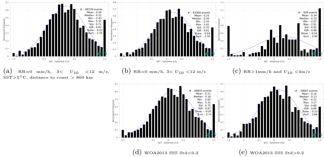
Figure 15: Normalized histogram of \Delta SSS (SMOS SSS L2Q v331 - No FLAG (CMEMS-CATDS-CPDC) - Sairdrone) for 5 different subdatasets corresponding to: RR=0 mm/h, 3 < U_{10} < 12 m/s, SST>5°C, distance to coast > 800 km (a), RR=0 mm/h, 3 < U_{10} < 12 m/s (b), RR>1mm/h and U_{10} < 4 m/s (c), WOA2013 SSS Std<0.2 (d), WOA2013 SSS Std>0.2 (e).
