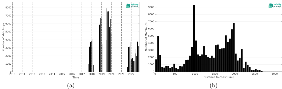
Figure 2: Number of match-ups between Saildrone and SMOS SSS L2Q v331 - No FLAG (CMEMS-CATDS-CPDC) SSS as a function of time (a) and as function of the distance to coast (b) over the Tropical Pacific Ocean Pi-MEP region and for the full satellite product period.
