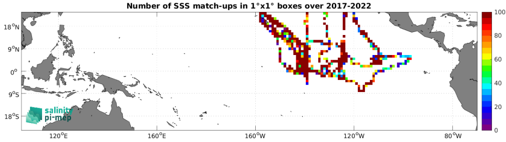
Figure 5: Number of SSS match-ups between Saildrone SSS and the SMOS SSS L2Q v331 - No FLAG (CMEMS-CATDS-CPDC) SSS product for the Tropical Pacific Ocean Pi-MEP region over 1^\circ \times 1^\circ boxes and for the full satellite product period.
