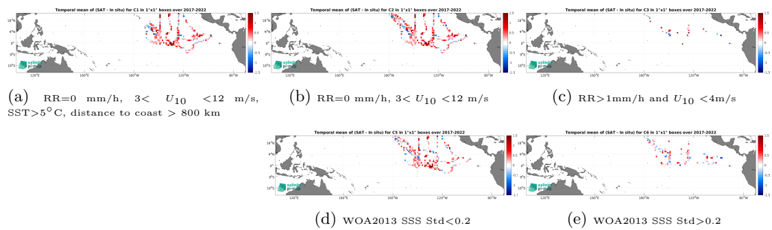
Figure 14: Temporal mean gridded over spatial boxes of size 1^\circ \times 1^\circ of \Delta\text{SSS} (SMOS SSS L2Q v331 - No FLAG (CMEMS-CATDS-CPDC) - Saildrone) for 5 different subdatasets corresponding to: RR=0 mm/h, 3 < U_{10} < 12 m/s, SST > 5°C, distance to coast > 800 km (a), RR=0 mm/h, 3 < U_{10} < 12 m/s (b), RR > 1mm/h and U_{10} < 4 m/s (c), WOA2013 SSS Std < 0.2 (d), WOA2013 SSS Std > 0.2 (e).
