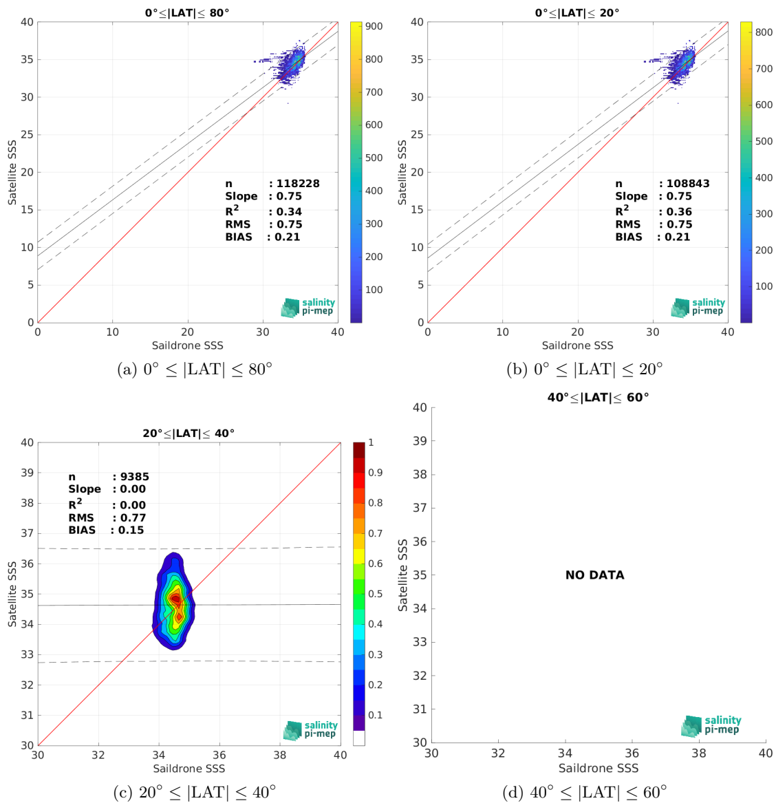
Figure 10: Contour maps of the concentration of SMOS SSS L2Q v331 - No FLAG (CMEMS-CATDS-CPDC) SSS (y-axis) versus Saildrone SSS (x-axis) at match-up pairs for different latitude bands. For each plot, the red line shows x=y . The black thin and dashed lines indicate a linear fit through the data cloud and the \pm 95\% confidence levels, respectively. The number match-up pairs n , the slope and R^2 coefficient of the linear fit, the root mean square (RMS) and the mean bias between satellite and in situ data are indicated for each latitude band in each plots.
