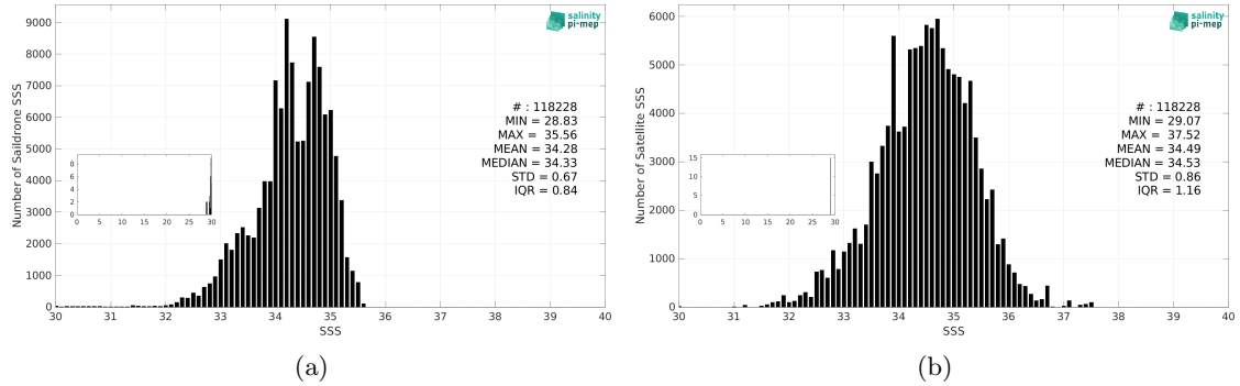
Figure 3: Histograms of SSS from Saildrone (a) and SMOS SSS L2Q v331 - No FLAG (CMEMS-CATDS-CPDC) (b) considering all match-up pairs per bins of 0.1 over the Tropical Pacific Ocean Pi-MEP region and for the full satellite product period.
