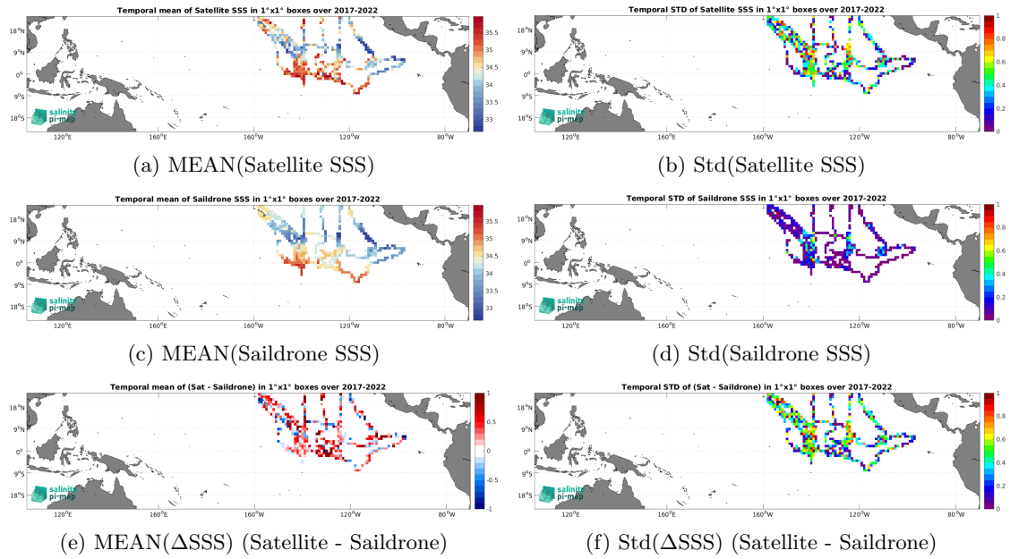
Figure 7: Temporal mean (left) and Std (right) of SSS from SMOS SSS L2Q v331 - No FLAG (CMEMS-CATDS-CPDC) (top), Saildrone (middle), and of \Delta SSS (Satellite - Saildrone). Only match-up pairs are used to generate these maps.
