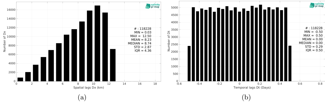
Figure 6: Histograms of the spatial (a) and temporal (b) lags between the location/time of the Saildrone measurement and the date of the corresponding SMOS SSS L2Q v331 - No FLAG (CMEMS-CATDS-CPDC) SSS pixel.
