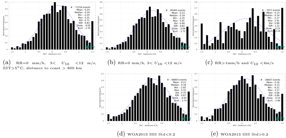
Figure 13: Normalized histogram of \Delta SSS (SMOS SSS L2Q v331 - No FLAG (CMEMS-CATDS-CPDC) - Sailsdrone) for 5 different subdatasets corresponding to: RR=0 mm/h, 3 < U_{10} < 12 m/s, SST>5°C, distance to coast > 800 km (a), RR=0 mm/h, 3 < U_{10} < 12 m/s (b), RR>1mm/h and U_{10} < 4 m/s (c), WOA2013 SSS Std<0.2 (d), WOA2013 SSS Std>0.2 (e).
