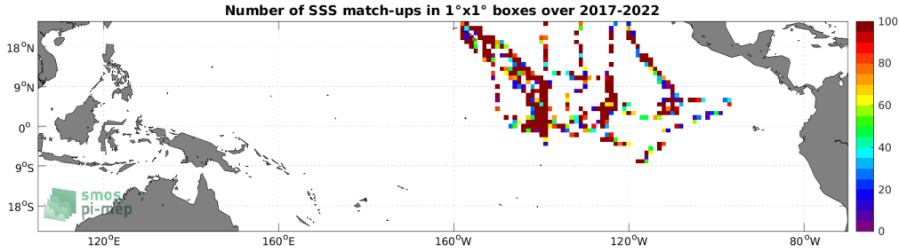
Figure 4: Number of SSS match-ups between Saildrone SSS and the SMOS SSS L2Q v331 - No FLAG (CMEMS-CATDS-CPDC) SSS product for the Tropical Pacific Ocean Pi-MEP region over 1^\circ \times 1^\circ boxes and for the full satellite product period.
