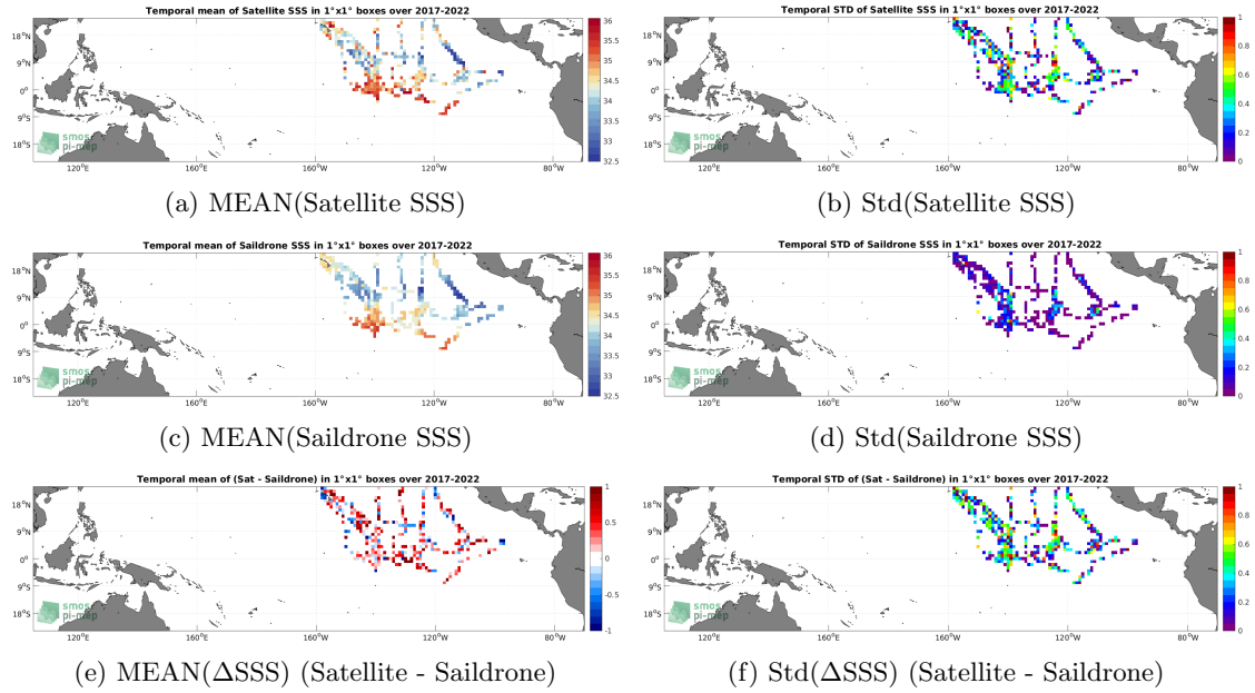
Figure 6: Temporal mean (left) and Std (right) of SSS from SMOS SSS L2Q v331 - No FLAG (CMEMS-CATDS-CPDC) (top), Saildrone (middle), and of \Delta SSS (Satellite - Saildrone). Only match-up pairs are used to generate these maps.
