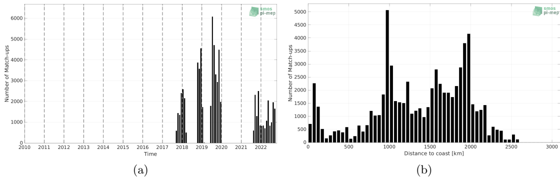
Figure 1: Number of match-ups between Saildrone and SMOS SSS L2Q v331 - No FLAG (CMEMS-CATDS-CPDC) SSS as a function of time (a) and as function of the distance to coast (b) over the Tropical Pacific Ocean Pi-MEP region and for the full satellite product period.
