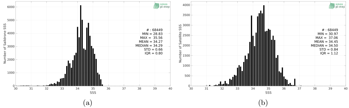
Figure 2: Histograms of SSS from Saildrone (a) and SMOS SSS L2Q v331 - No FLAG (CMEMS-CATDS-CPDC) (b) considering all match-up pairs per bins of 0.1 over the Tropical Pacific Ocean Pi-MEP region and for the full satellite product period.
