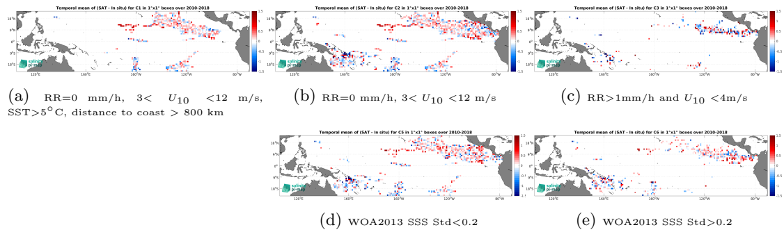
Figure 13: Temporal mean gridded over spatial boxes of size 1^\circ \times 1^\circ of \Delta SSS (SMOS SSS L2Q v331 - No FLAG (CMEMS-CATDS-CPDC) - Surface drifters) for 5 different subdatasets corresponding to:RR=0 mm/h, 3 < U_{10} < 12 m/s, SST > 5^\circ\text{C} , distance to coast > 800 km (a), RR=0 mm/h, 3 < U_{10} < 12 m/s (b), RR > 1 mm/h and U_{10} < 4 m/s (c), WOA2013 SSS Std < 0.2 (d), WOA2013 SSS Std > 0.2 (e).
