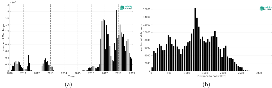
Figure 2: Number of match-ups between Surface drifters and SMOS SSS L2Q v331 - No FLAG (CMEMS-CATDS-CPDC) SSS as a function of time (a) and as function of the distance to coast (b) over the Tropical Pacific Ocean Pi-MEP region and for the full satellite product period.
