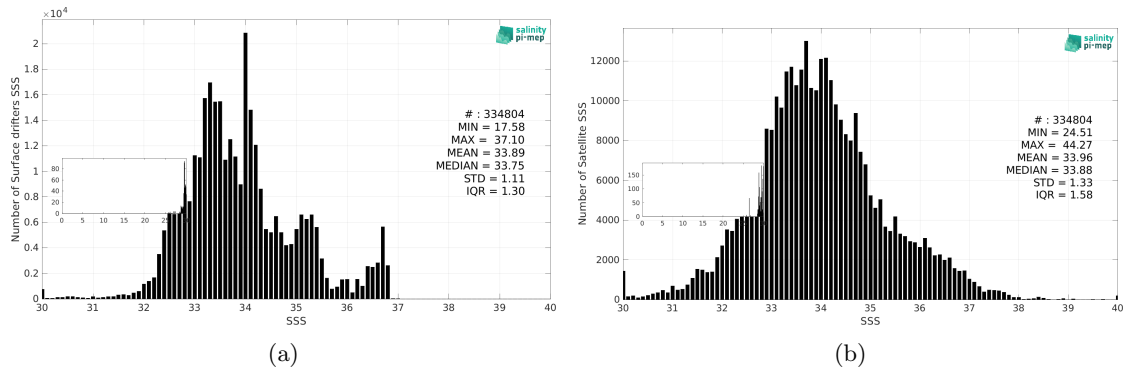
Figure 3: Histograms of SSS from Surface drifters (a) and SMOS SSS L2Q v331 - No FLAG (CMEMS-CATDS-CPDC) (b) considering all match-up pairs per bins of 0.1 over the Tropical Pacific Ocean Pi-MEP region and for the full satellite product period.
