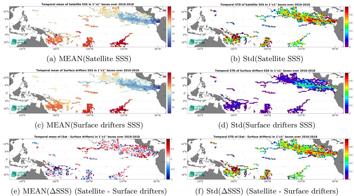
Figure 6: Temporal mean (left) and Std (right) of SSS from SMOS SSS L2Q v331 - No FLAG (CMEMS-CATDS-CPDC) (top), Surface drifters (middle), and of \Delta SSS (Satellite - Surface drifters). Only match-up pairs are used to generate these maps.
