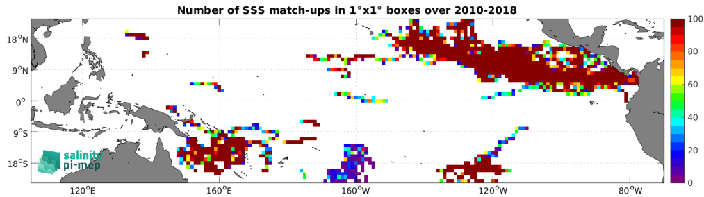
Figure 4: Number of SSS match-ups between Surface drifters SSS and the SMOS SSS L2Q v331 - No FLAG (CMEMS-CATDS-CPDC) SSS product for the Tropical Pacific Ocean Pi-MEP region over 1^\circ \times 1^\circ boxes and for the full satellite product period.
