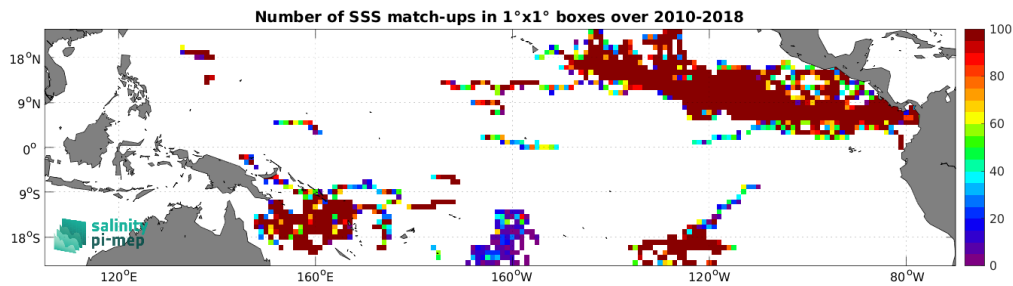
Figure 3: Number of SSS match-ups between Surface drifters SSS and the SMOS SSS L2Q v331 - No FLAG (CMEMS-CATDS-CPDC) SSS product for the Tropical Pacific Ocean Pi-MEP region over 1^\circ \times 1^\circ boxes and for the full satellite product period.
