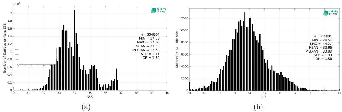
Figure 2: Histograms of SSS from Surface drifters (a) and SMOS SSS L2Q v331 - No FLAG (CMEMS-CATDS-CPDC) (b) considering all match-up pairs per bins of 0.1 over the Tropical Pacific Ocean Pi-MEP region and for the full satellite product period.
