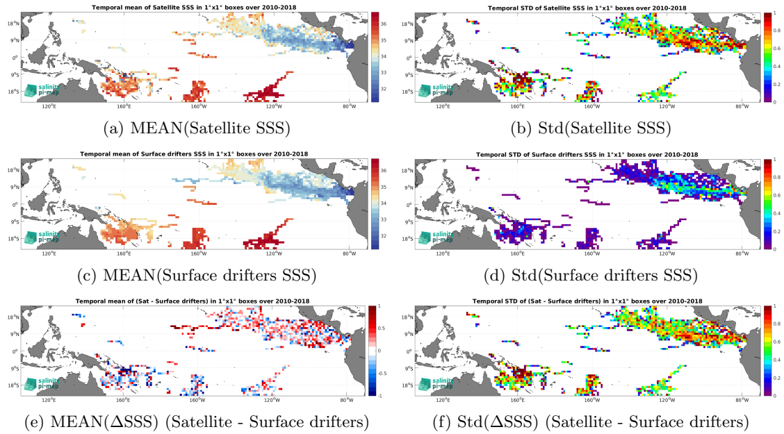
Figure 5: Temporal mean (left) and Std (right) of SSS from SMOS SSS L2Q v331 - No FLAG (CMEMS-CATDS-CPDC) (top), Surface drifters (middle), and of \Delta SSS (Satellite - Surface drifters). Only match-up pairs are used to generate these maps.
