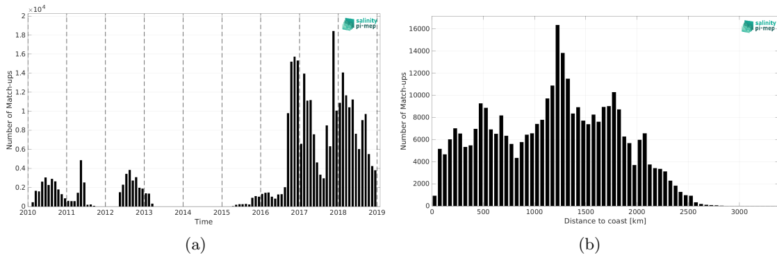
Figure 1: Number of match-ups between Surface drifters and SMOS SSS L2Q v331 - No FLAG (CMEMS-CATDS-CPDC) SSS as a function of time (a) and as function of the distance to coast (b) over the Tropical Pacific Ocean Pi-MEP region and for the full satellite product period.
