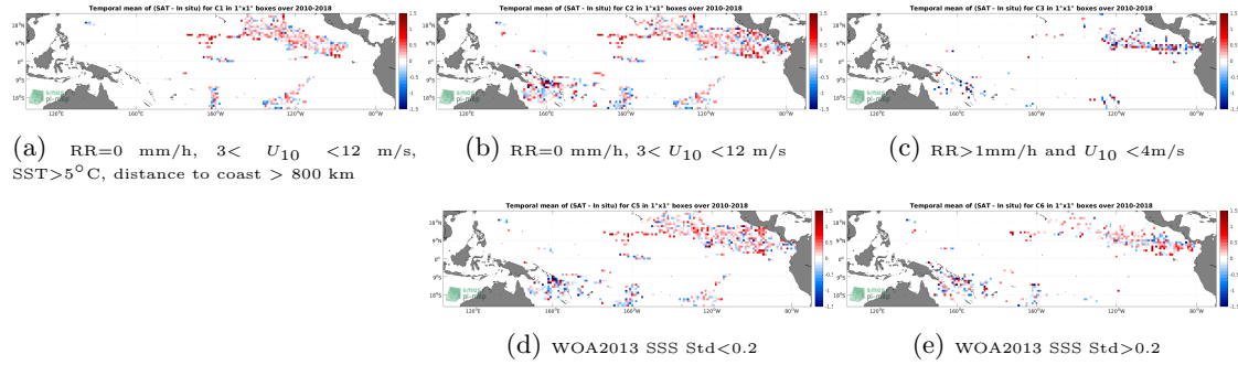
Figure 11: Temporal mean gridded over spatial boxes of size 1^{\circ}\times 1^{\circ} of \Delta\text{SSS} (SMOS SSS L2Q v331 - No FLAG (CMEMS-CATDS-CPDC) - Surface drifters) for 5 different subdatasets corresponding to:RR=0 mm/h, 3 < U_{10} < 12 m/s, SST > 5^{\circ}\text{C} , distance to coast > 800 km (a), RR=0 mm/h, 3 < U_{10} < 12 m/s (b), RR > 1 mm/h and U_{10} < 4 m/s (c), WOA2013 SSS Std < 0.2 (d), WOA2013 SSS Std > 0.2 (e).
