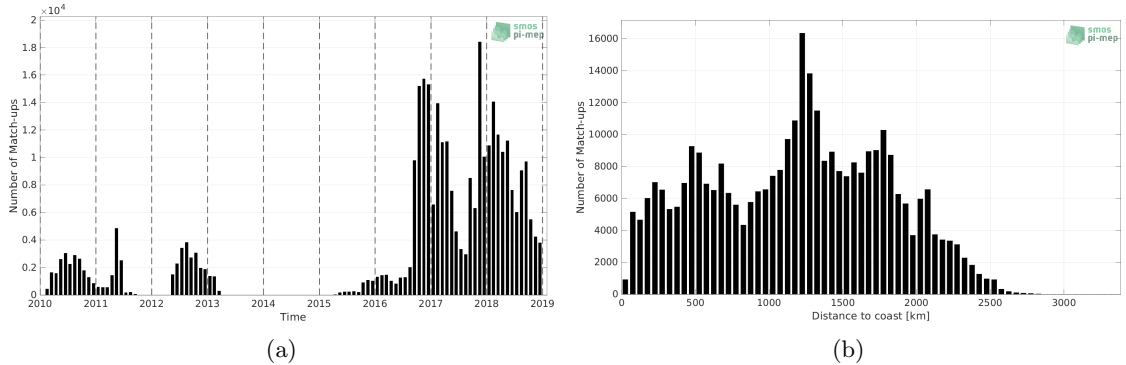
Figure 1: Number of match-ups between Surface drifters and SMOS SSS L2Q v331 - No FLAG (CMEMS-CATDS-CPDC) SSS as a function of time (a) and as function of the distance to coast (b) over the Tropical Pacific Ocean Pi-MEP region and for the full satellite product period.
