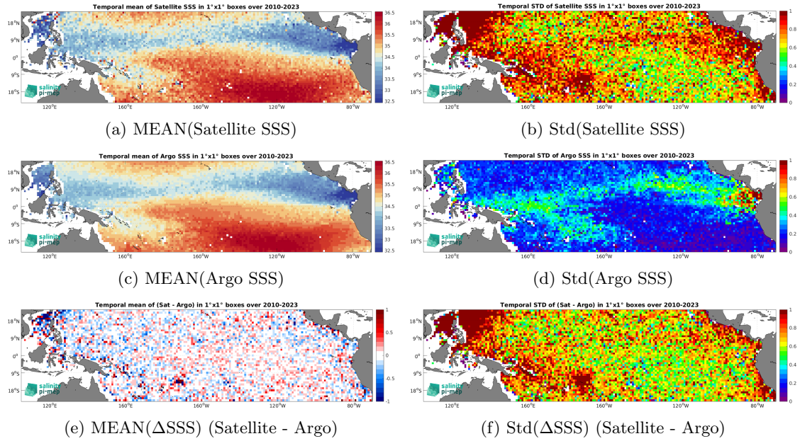
Figure 6: Temporal mean (left) and Std (right) of SSS from SMOS SSS L2Q v331 - No FLAG (CMEMS-CATDS-CPDC) (top), Argo (middle), and of \Delta SSS (Satellite - Argo). Only match-up pairs are used to generate these maps.
