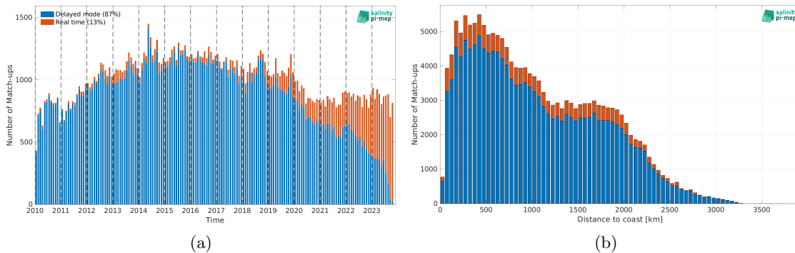
Figure 1: Number of match-ups between Argo and SMOS SSS L2Q v331 - No FLAG (CMEMS-CATDS-CPDC) SSS as a function of time (a) and as function of the distance to coast (b) over the Tropical Pacific Ocean Pi-MEP region and for the full satellite product period.
