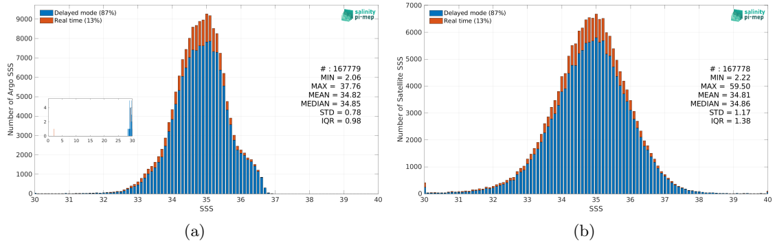
Figure 2: Histograms of SSS from Argo (a) and SMOS SSS L2Q v331 - No FLAG (CMEMS-CATDS-CPDC) (b) considering all match-up pairs per bins of 0.1 over the Tropical Pacific Ocean Pi-MEP region and for the full satellite product period.
