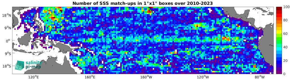
Figure 4: Number of SSS match-ups between Argo SSS and the SMOS SSS L2Q v331 - No FLAG (CMEMS-CATDS-CPDC) SSS product for the Tropical Pacific Ocean Pi-MEP region over 1^\circ \times 1^\circ boxes and for the full satellite product period.
