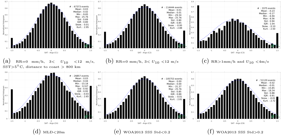
Figure 13: Normalized histogram of \Delta\text{SSS} (SMOS SSS L2Q v331 - No FLAG (CMEMS-CATDS-CPDC) - Argo) for 6 different subdatasets corresponding to: RR=0 mm/h, 3 < U_{10} < 12 m/s, SST>5°C, distance to coast > 800 km (a), RR=0 mm/h, 3 < U_{10} < 12 m/s (b), RR>1mm/h and U_{10} < 4 m/s (c), MLD<20m (d), WOA2013 SSS Std<0.2 (e), WOA2013 SSS Std>0.2 (f).
