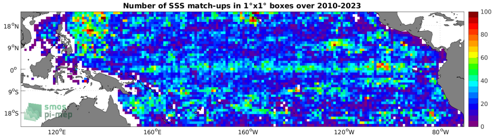
Figure 4: Number of SSS match-ups between Argo SSS and the SMOS SSS L2Q v331 - No FLAG (CMEMS-CATDS-CPDC) SSS product for the Tropical Pacific Ocean Pi-MEP region over 1^\circ \times 1^\circ boxes and for the full satellite product period.
