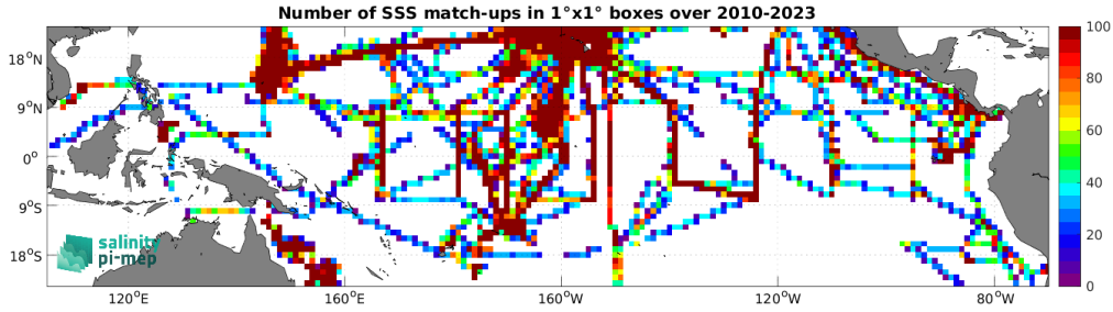
Figure 5: Number of SSS match-ups between TSG (SAMOS) SSS and the SMOS SSS L3 v9 - 9 Days (CATDS-CEC-LOCEAN) SSS product for the Tropical Pacific Ocean Pi-MEP region over 1^\circ \times 1^\circ boxes and for the full satellite product period.
