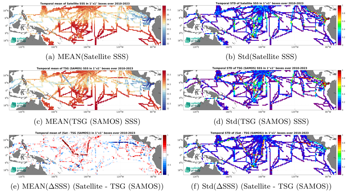
Figure 7: Temporal mean (left) and Std (right) of SSS from SMOS SSS L3 v9 - 9 Days (CATDS-CEC-LOCEAN) (top), TSG (SAMOS) (middle), and of \Delta SSS (Satellite - TSG (SAMOS)). Only match-up pairs are used to generate these maps.
