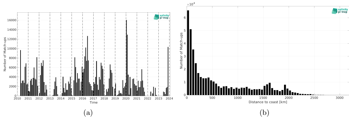
Figure 2: Number of match-ups between TSG (SAMOS) and SMOS SSS L3 v9 - 9 Days (CATDS-CEC-LOCEAN) SSS as a function of time (a) and as function of the distance to coast (b) over the Tropical Pacific Ocean Pi-MEP region and for the full satellite product period.
