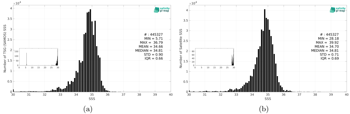
Figure 3: Histograms of SSS from TSG (SAMOS) (a) and SMOS SSS L3 v9 - 9 Days (CATDS-CEC-LOCEAN) (b) considering all match-up pairs per bins of 0.1 over the Tropical Pacific Ocean Pi-MEP region and for the full satellite product period.
