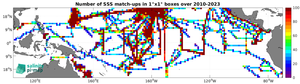
Figure 4: Number of SSS match-ups between TSG (SAMOS) SSS and the SMOS SSS L3 v9 - 9 Days (CATDS-CEC-LOCEAN) SSS product for the Tropical Pacific Ocean Pi-MEP region over 1^\circ \times 1^\circ boxes and for the full satellite product period.
