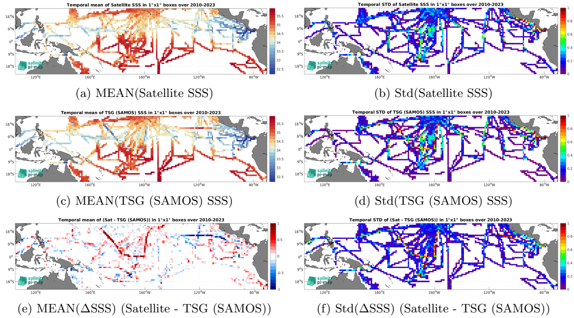
Figure 6: Temporal mean (left) and Std (right) of SSS from SMOS SSS L3 v9 - 9 Days (CATDS-CEC-LOCEAN) (top), TSG (SAMOS) (middle), and of \Delta SSS (Satellite - TSG (SAMOS)). Only match-up pairs are used to generate these maps.
