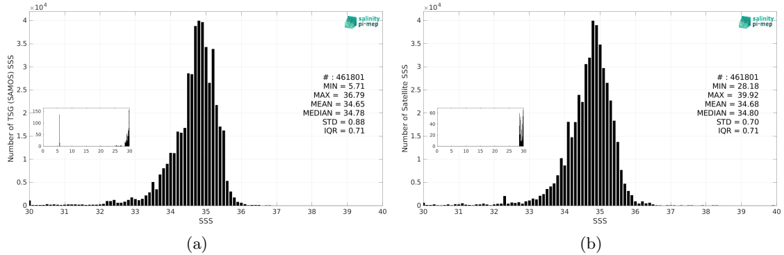
Figure 2: Histograms of SSS from TSG (SAMOS) (a) and SMOS SSS L3 v9 - 9 Days (CATDS-CEC-LOCEAN) (b) considering all match-up pairs per bins of 0.1 over the Tropical Pacific Ocean Pi-MEP region and for the full satellite product period.
