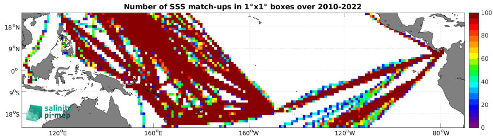
Figure 5: Number of SSS match-ups between TSG (LEGOS-DM) SSS and the SMOS SSS L3 v9 - 9 Days (CATDS-CEC-LOCEAN) SSS product for the Tropical Pacific Ocean Pi-MEP region over 1^\circ \times 1^\circ boxes and for the full satellite product period.
