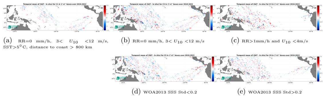
Figure 14: Temporal mean gridded over spatial boxes of size 1^\circ \times 1^\circ of \Delta SSS (SMOS SSS L3 v9 - 9 Days (CATDS-CEC-LOCEAN) - TSG (LEGOS-DM)) for 5 different subdatasets corresponding to: RR=0 mm/h, 3 < U_{10} < 12 m/s, SST > 5^\circ\text{C} , distance to coast > 800 km (a), RR=0 mm/h, 3 < U_{10} < 12 m/s (b), RR > 1 mm/h and U_{10} < 4 m/s (c), WOA2013 SSS Std < 0.2 (d), WOA2013 SSS Std > 0.2 (e).
