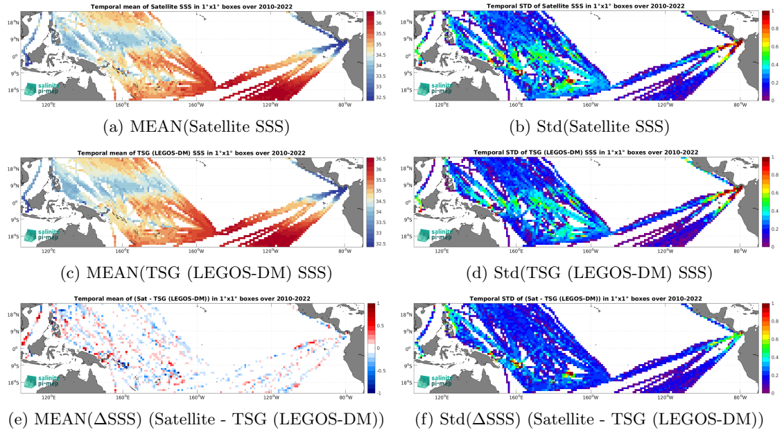
Figure 7: Temporal mean (left) and Std (right) of SSS from SMOS SSS L3 v9 - 9 Days (CATDS-CEC-LOCEAN) (top), TSG (LEGOS-DM) (middle), and of \Delta SSS (Satellite - TSG (LEGOS-DM)). Only match-up pairs are used to generate these maps.
