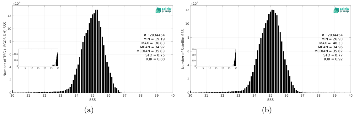
Figure 3: Histograms of SSS from TSG (LEGOS-DM) (a) and SMOS SSS L3 v9 - 9 Days (CATDS-CEC-LOCEAN) (b) considering all match-up pairs per bins of 0.1 over the Tropical Pacific Ocean Pi-MEP region and for the full satellite product period.
