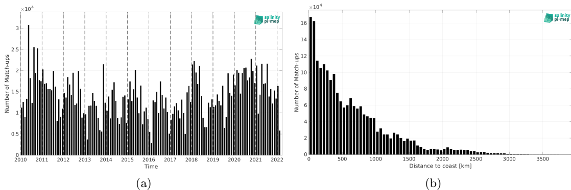
Figure 2: Number of match-ups between TSG (LEGOS-DM) and SMOS SSS L3 v9 - 9 Days (CATDS-CEC-LOCEAN) SSS as a function of time (a) and as function of the distance to coast (b) over the Tropical Pacific Ocean Pi-MEP region and for the full satellite product period.
