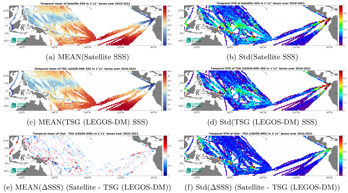
Figure 6: Temporal mean (left) and Std (right) of SSS from SMOS SSS L3 v9 - 9 Days (CATDS-CEC-LOCEAN) (top), TSG (LEGOS-DM) (middle), and of \Delta SSS (Satellite - TSG (LEGOS-DM)). Only match-up pairs are used to generate these maps.
