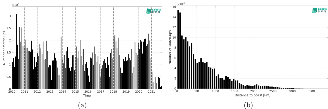
Figure 1: Number of match-ups between TSG (LEGOS-DM) and SMOS SSS L3 v9 - 9 Days (CATDS-CEC-LOCEAN) SSS as a function of time (a) and as function of the distance to coast (b) over the Tropical Pacific Ocean Pi-MEP region and for the full satellite product period.
