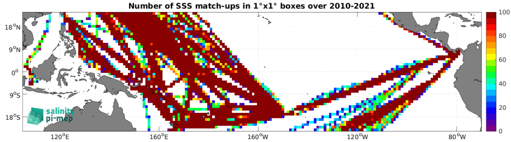
Figure 4: Number of SSS match-ups between TSG (LEGOS-DM) SSS and the SMOS SSS L3 v9 - 9 Days (CATDS-CEC-LOCEAN) SSS product for the Tropical Pacific Ocean Pi-MEP region over 1^\circ \times 1^\circ boxes and for the full satellite product period.
