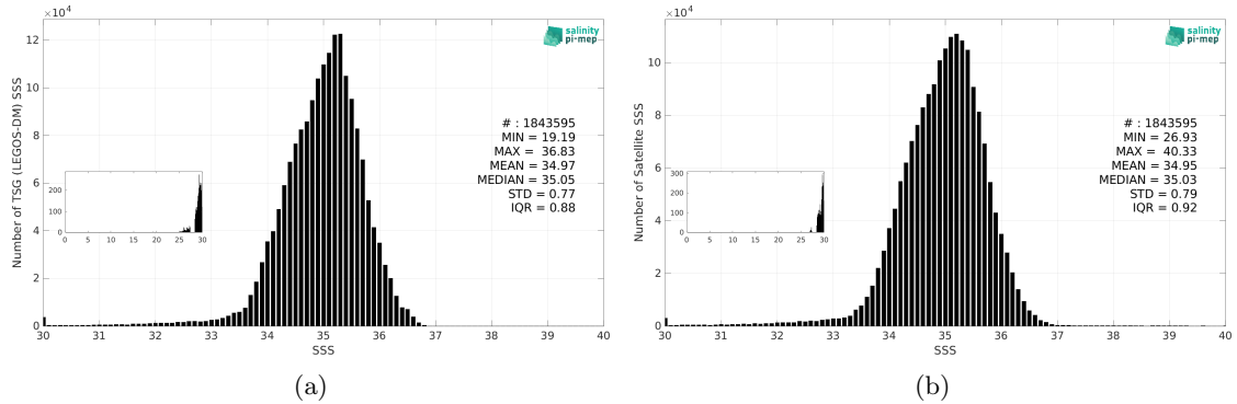
Figure 2: Histograms of SSS from TSG (LEGOS-DM) (a) and SMOS SSS L3 v9 - 9 Days (CATDS-CEC-LOCEAN) (b) considering all match-up pairs per bins of 0.1 over the Tropical Pacific Ocean Pi-MEP region and for the full satellite product period.
