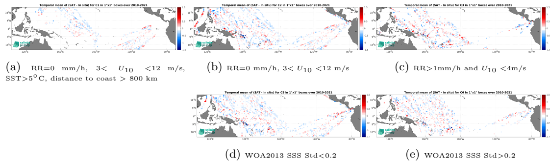
Figure 12: Temporal mean gridded over spatial boxes of size 1^{\circ}\times 1^{\circ} of \Delta\text{SSS} (SMOS SSS L3 v9 - 9 Days (CATDS-CEC-LOCEAN) - TSG (LEGOS-DM)) for 5 different subdatasets corresponding to:RR=0 mm/h, 3 < U_{10} < 12 m/s, SST >5^{\circ}\text{C} , distance to coast > 800 km (a), RR=0 mm/h, 3 < U_{10} < 12 m/s (b), RR >1 mm/h and U_{10} < 4 m/s (c), WOA2013 SSS Std <0.2 (d), WOA2013 SSS Std >0.2 (e).
