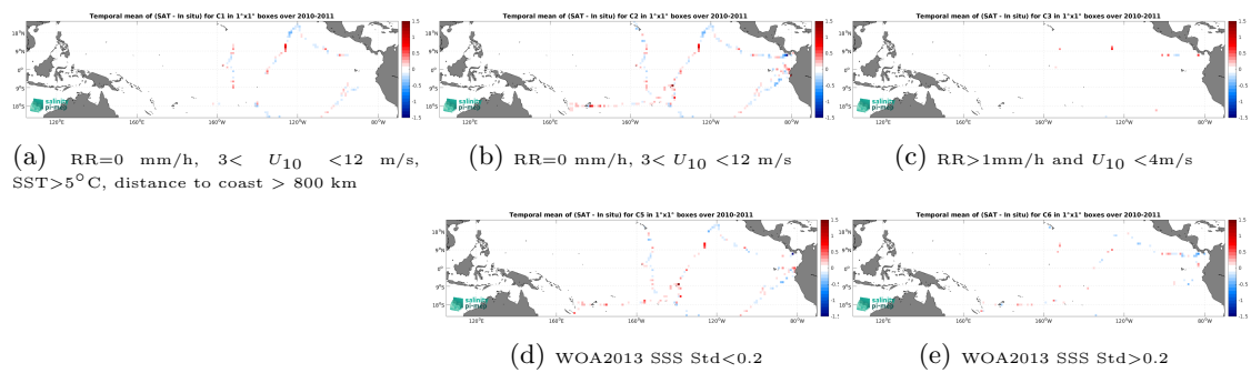
Figure 14: Temporal mean gridded over spatial boxes of size 1^\circ \times 1^\circ of \Delta SSS (SMOS SSS L3 v9 - 9 Days (CATDS-CEC-LOCEAN) - TSG (GOSUD-Sailing-ship)) for 5 different subdatasets corresponding to:RR=0 mm/h, 3 < U_{10} < 12 m/s, SST >5^\circ\text{C} , distance to coast > 800 km (a), RR=0 mm/h, 3 < U_{10} < 12 m/s (b), RR >1 mm/h and U_{10} < 4 m/s (c), WOA2013 SSS Std <0.2 (d), WOA2013 SSS Std >0.2 (e).
