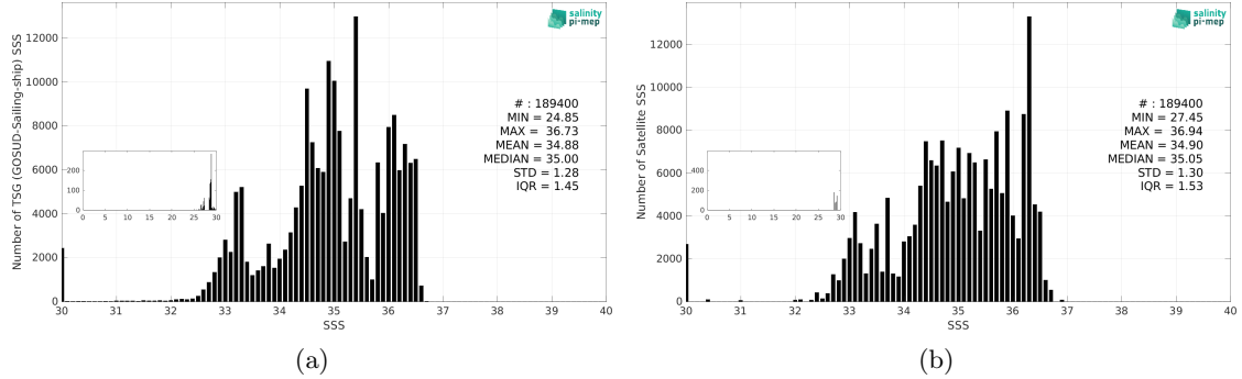
Figure 3: Histograms of SSS from TSG (GOSUD-Sailing-ship) (a) and SMOS SSS L3 v9 - 9 Days (CATDS-CEC-LOCEAN) (b) considering all match-up pairs per bins of 0.1 over the Tropical Pacific Ocean Pi-MEP region and for the full satellite product period.
