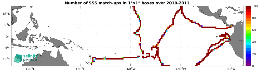
Figure 5: Number of SSS match-ups between TSG (GOSUD-Sailing-ship) SSS and the SMOS SSS L3 v9 - 9 Days (CATDS-CEC-LOCEAN) SSS product for the Tropical Pacific Ocean Pi-MEP region over 1^\circ \times 1^\circ boxes and for the full satellite product period.
