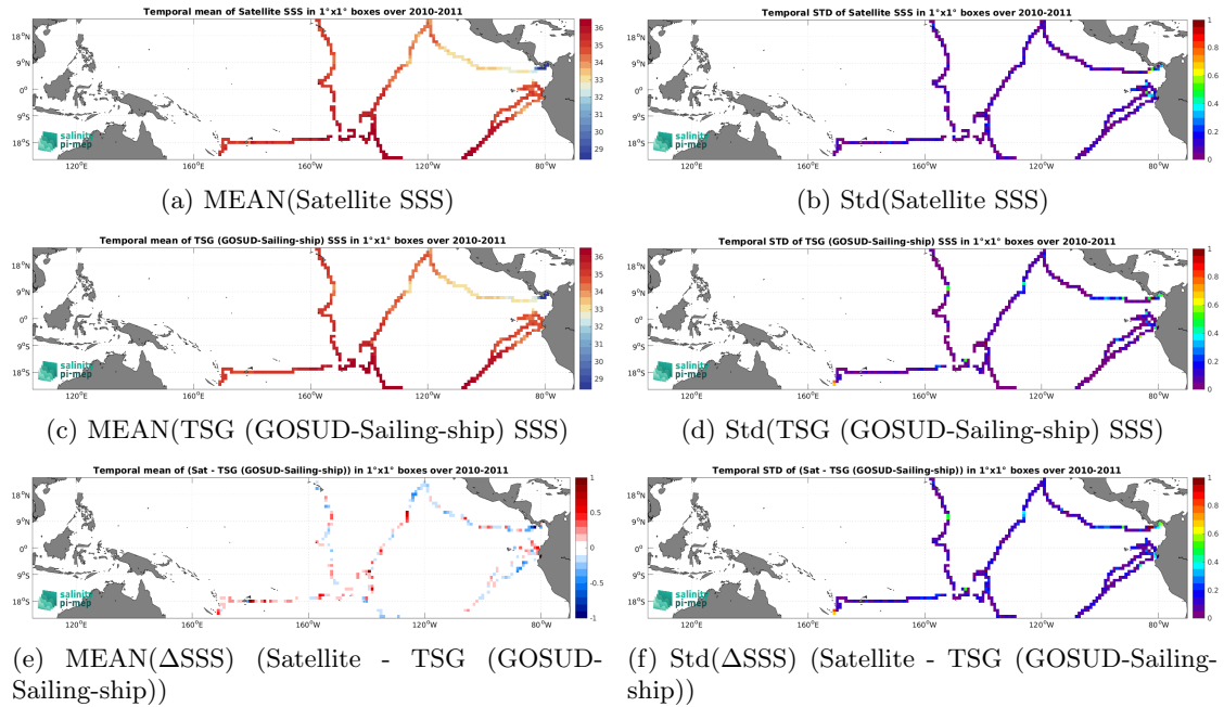
Figure 6: Temporal mean (left) and Std (right) of SSS from SMOS SSS L3 v9 - 9 Days (CATDS-CEC-LOCEAN) (top), TSG (GOSUD-Sailing-ship) (middle), and of \Delta SSS (Satellite - TSG (GOSUD-Sailing-ship)). Only match-up pairs are used to generate these maps.
