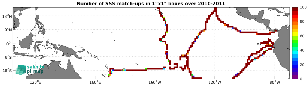
Figure 4: Number of SSS match-ups between TSG (GOSUD-Sailing-ship) SSS and the SMOS SSS L3 v9 - 9 Days (CATDS-CEC-LOCEAN) SSS product for the Tropical Pacific Ocean Pi-MEP region over 1^\circ \times 1^\circ boxes and for the full satellite product period.
