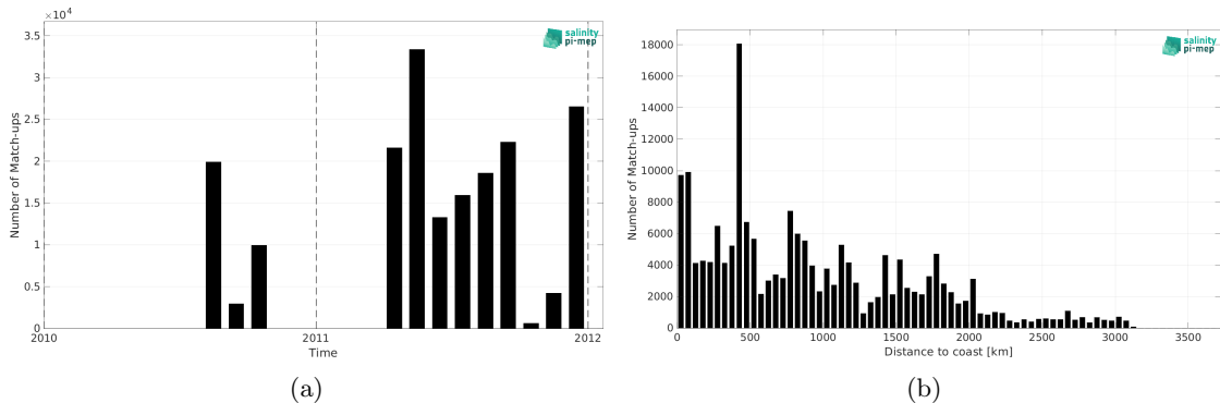
Figure 1: Number of match-ups between TSG (GOSUD-Sailing-ship) and SMOS SSS L3 v9 - 9 Days (CATDS-CEC-LOCEAN) SSS as a function of time (a) and as function of the distance to coast (b) over the Tropical Pacific Ocean Pi-MEP region and for the full satellite product period.
