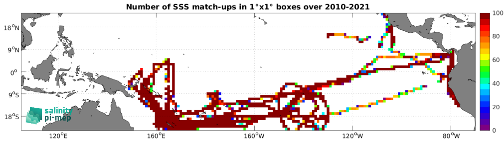
Figure 5: Number of SSS match-ups between TSG (GOSUD-Research-vessel) SSS and the SMOS SSS L3 v9 - 9 Days (CATDS-CEC-LOCEAN) SSS product for the Tropical Pacific Ocean Pi-MEP region over 1^\circ \times 1^\circ boxes and for the full satellite product period.
