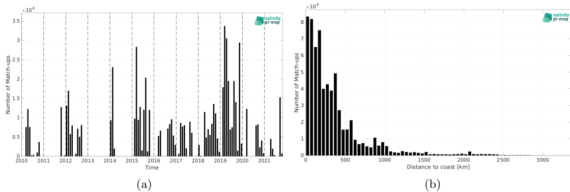
Figure 2: Number of match-ups between TSG (GOSUD-Research-vessel) and SMOS SSS L3 v9 - 9 Days (CATDS-CEC-LOCEAN) SSS as a function of time (a) and as function of the distance to coast (b) over the Tropical Pacific Ocean Pi-MEP region and for the full satellite product period.
