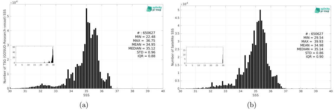
Figure 3: Histograms of SSS from TSG (GOSUD-Research-vessel) (a) and SMOS SSS L3 v9 - 9 Days (CATDS-CEC-LOCEAN) (b) considering all match-up pairs per bins of 0.1 over the Tropical Pacific Ocean Pi-MEP region and for the full satellite product period.
