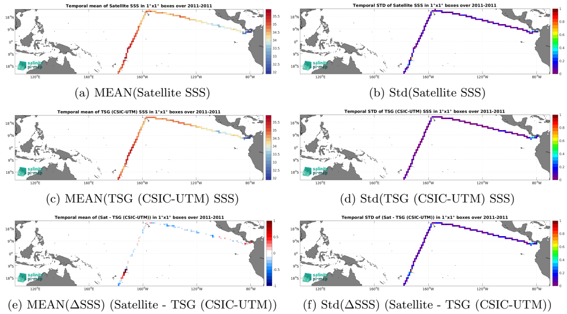
Figure 7: Temporal mean (left) and Std (right) of SSS from SMOS SSS L3 v9 - 9 Days (CATDS-CEC-LOCEAN) (top), TSG (CSIC-UTM) (middle), and of \Delta SSS (Satellite - TSG (CSIC-UTM)). Only match-up pairs are used to generate these maps.
