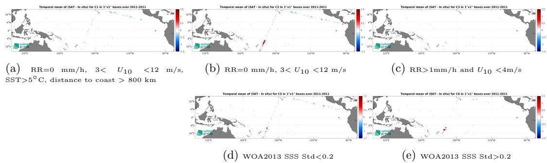
Figure 14: Temporal mean gridded over spatial boxes of size 1^\circ \times 1^\circ of \Delta SSS (SMOS SSS L3 v9 - 9 Days (CATDS-CEC-LOCEAN) - TSG (CSIC-UTM)) for 5 different subdatasets corresponding to:RR=0 mm/h, 3 < U_{10} < 12 m/s, SST >5^\circ\text{C} , distance to coast > 800 km (a), RR=0 mm/h, 3 < U_{10} < 12 m/s (b), RR >1 mm/h and U_{10} < 4 m/s (c), WOA2013 SSS Std <0.2 (d), WOA2013 SSS Std >0.2 (e).
