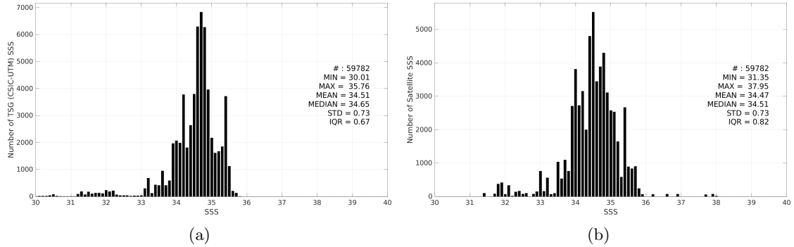
Figure 3: Histograms of SSS from TSG (CSIC-UTM) (a) and SMOS SSS L3 v9 - 9 Days (CATDS-CEC-LOCEAN) (b) considering all match-up pairs per bins of 0.1 over the Tropical Pacific Ocean Pi-MEP region and for the full satellite product period.
