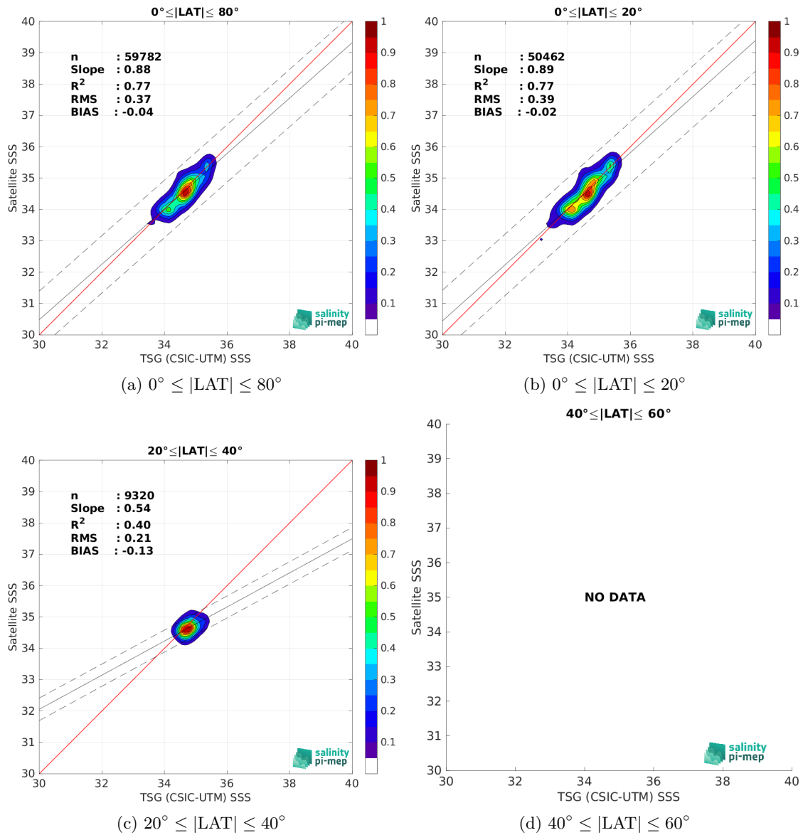
Figure 9: Contour maps of the concentration of SMOS SSS L3 v9 - 9 Days (CATDS-CEC-LOCEAN) SSS (y-axis) versus TSG (CSIC-UTM) SSS (x-axis) at match-up pairs for different latitude bands. For each plot, the red line shows x=y . The black thin and dashed lines indicate a linear fit through the data cloud and the \pm 95\% confidence levels, respectively. The number match-up pairs n , the slope and R^2 coefficient of the linear fit, the root mean square (RMS) and the mean bias between satellite and in situ data are indicated for each latitude band in each plots.
