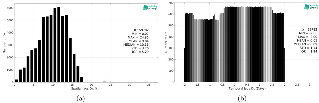
Figure 5: Histograms of the spatial (a) and temporal (b) lags between the location/time of the TSG (CSIC-UTM) measurement and the date of the corresponding SMOS SSS L3 v9 - 9 Days (CATDS-CEC-LOCEAN) SSS pixel.
