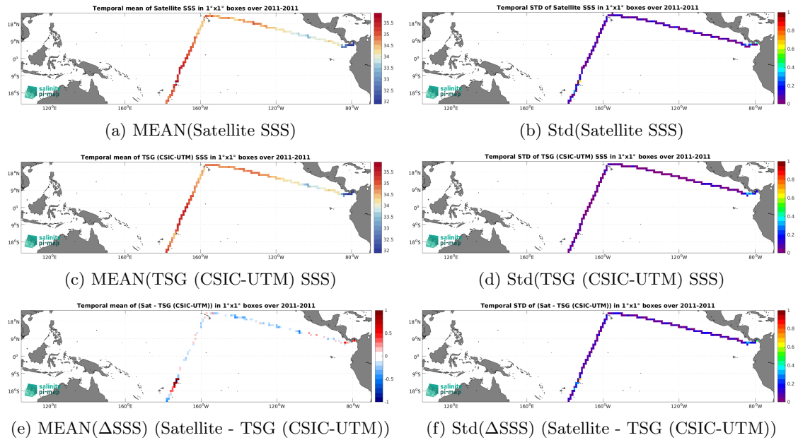
Figure 6: Temporal mean (left) and Std (right) of SSS from SMOS SSS L3 v9 - 9 Days (CATDS-CEC-LOCEAN) (top), TSG (CSIC-UTM) (middle), and of \Delta SSS (Satellite - TSG (CSIC-UTM)). Only match-up pairs are used to generate these maps.
