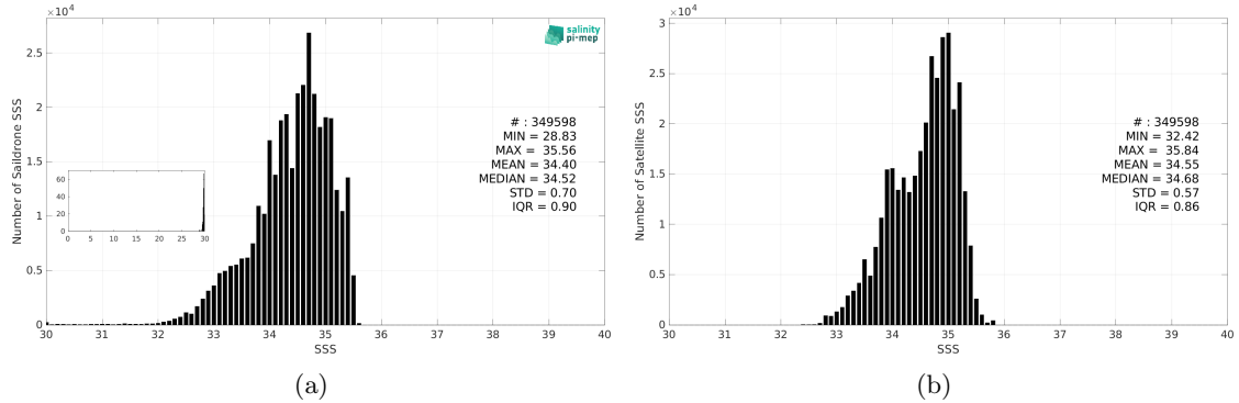
Figure 3: Histograms of SSS from Saildrone (a) and SMOS SSS L3 v9 - 9 Days (CATDS-CEC-LOCEAN) (b) considering all match-up pairs per bins of 0.1 over the Tropical Pacific Ocean Pi-MEP region and for the full satellite product period.
