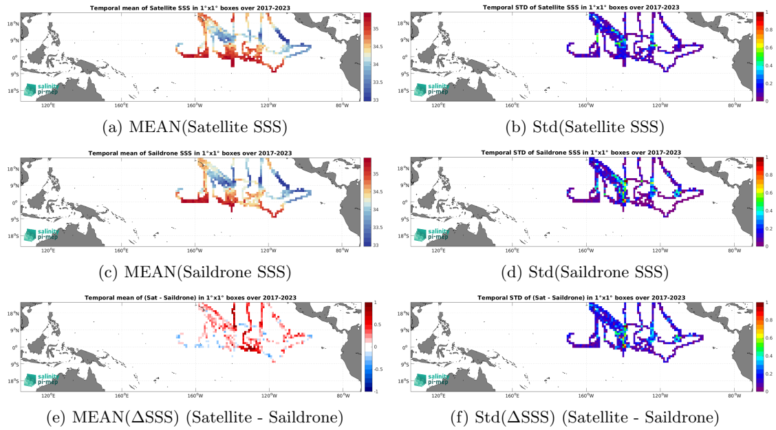
Figure 7: Temporal mean (left) and Std (right) of SSS from SMOS SSS L3 v9 - 9 Days (CATDS-CEC-LOCEAN) (top), Saildrone (middle), and of \Delta SSS (Satellite - Saildrone). Only match-up pairs are used to generate these maps.
