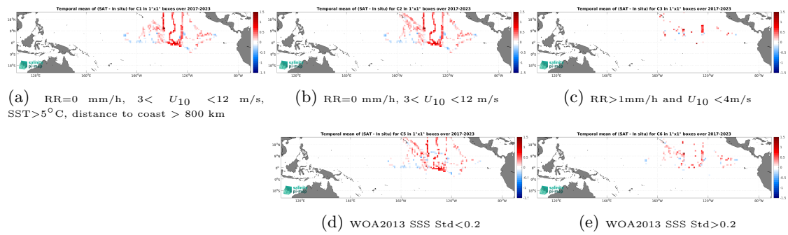
Figure 14: Temporal mean gridded over spatial boxes of size 1^\circ \times 1^\circ of \Delta SSS (SMOS SSS L3 v9 - 9 Days (CATDS-CEC-LOCEAN) - Saldrone) for 5 different subdatasets corresponding to:RR=0 mm/h, 3 < U_{10} < 12 m/s, SST >5^\circ C, distance to coast > 800 km (a), RR=0 mm/h, 3 < U_{10} < 12 m/s (b), RR >1 mm/h and U_{10} < 4 m/s (c), WOA2013 SSS Std <0.2 (d), WOA2013 SSS Std >0.2 (e).
