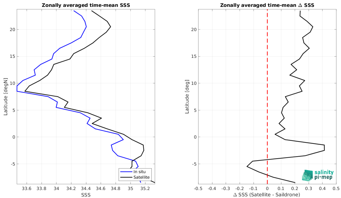
Figure 9: Left panel: Zonal mean SSS from SMOS SSS L3 v9 - 9 Days (CATDS-CEC-LOCEAN) satellite product (black) and from Saildrone (blue). Right panel: Zonal mean of \Delta SSS (Satellite - Saildrone) for all the collected Pi-MEP match-up pairs estimated over the full satellite product period.
