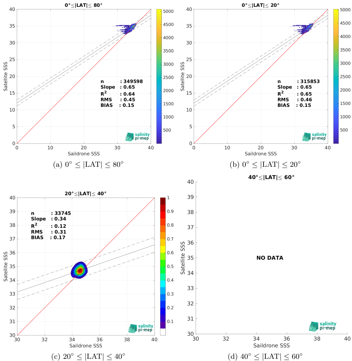
Figure 10: Contour maps of the concentration of SMOS SSS L3 v9 - 9 Days (CATDS-CEC-LOCEAN) SSS (y-axis) versus Sairdrone SSS (x-axis) at match-up pairs for different latitude bands. For each plot, the red line shows x=y . The black thin and dashed lines indicate a linear fit through the data cloud and the \pm 95\% confidence levels, respectively. The number match-up pairs n , the slope and R^2 coefficient of the linear fit, the root mean square (RMS) and the mean bias between satellite and in situ data are indicated for each latitude band in each plots.
