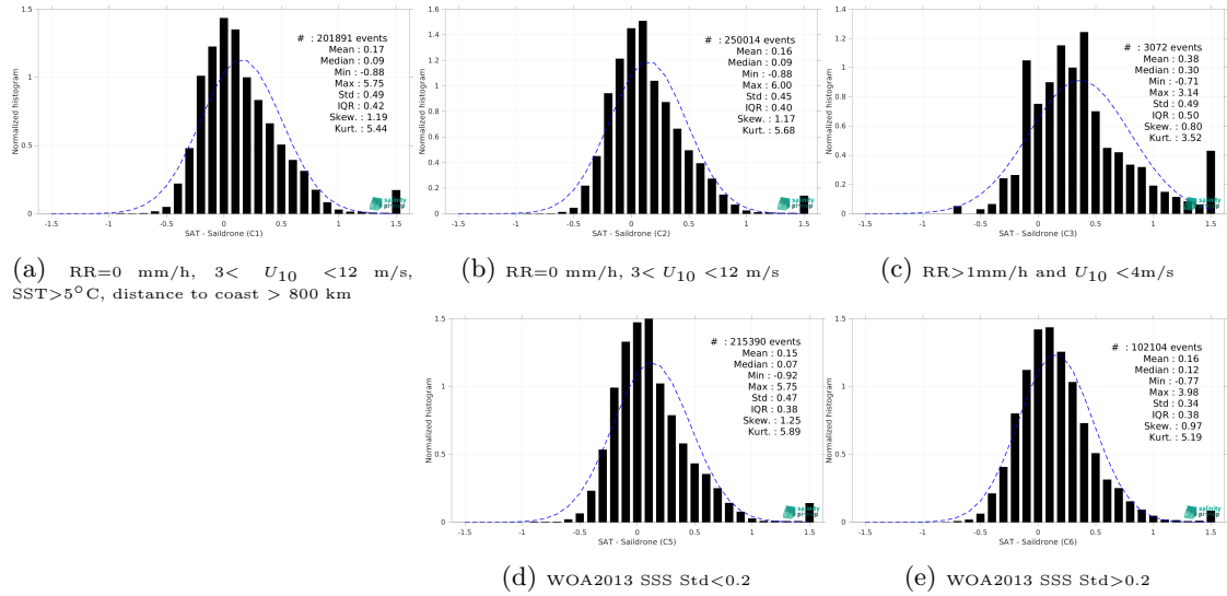
Figure 15: Normalized histogram of \Delta SSS (SMOS SSS L3 v9 - 9 Days (CATDS-CEC-LOCEAN) - Saildrone) for 5 different subdatasets corresponding to: RR=0 mm/h, 3 < U_{10} < 12 m/s, SST>5°C, distance to coast > 800 km (a), RR=0 mm/h, 3 < U_{10} < 12 m/s (b), RR>1mm/h and U_{10} < 4 m/s (c), WOA2013 SSS Std<0.2 (d), WOA2013 SSS Std>0.2 (e).
