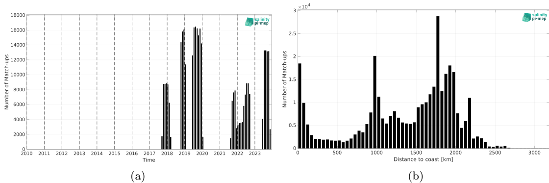
Figure 2: Number of match-ups between Saildrone and SMOS SSS L3 v9 - 9 Days (CATDS-CEC-LOCEAN) SSS as a function of time (a) and as function of the distance to coast (b) over the Tropical Pacific Ocean Pi-MEP region and for the full satellite product period.
