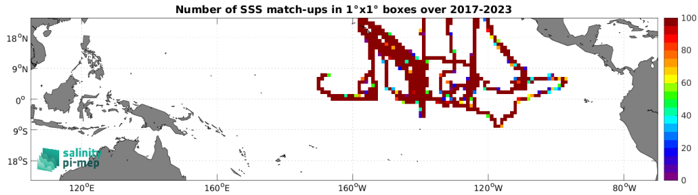
Figure 5: Number of SSS match-ups between Saildrone SSS and the SMOS SSS L3 v9 - 9 Days (CATDS-CEC-LOCEAN) SSS product for the Tropical Pacific Ocean Pi-MEP region over 1^\circ \times 1^\circ boxes and for the full satellite product period.
