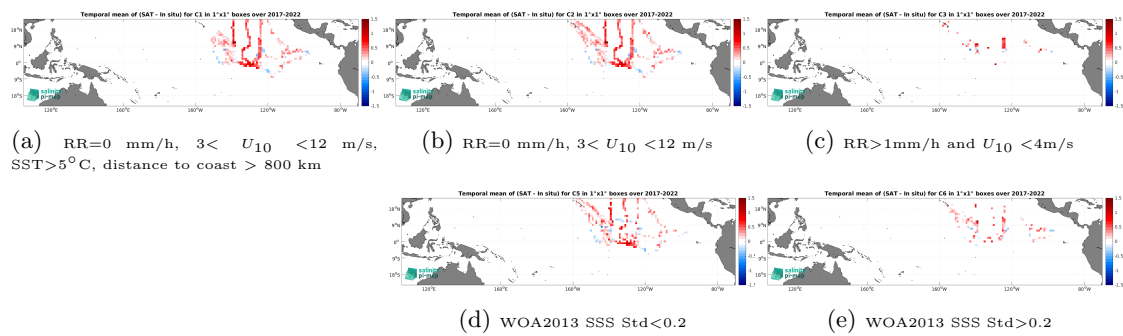
Figure 14: Temporal mean gridded over spatial boxes of size 1^\circ \times 1^\circ of \Delta SSS (SMOS SSS L3 v9 - 9 Days (CATDS-CEC-LOCEAN) - Saildrone) for 5 different subdatasets corresponding to:RR=0 mm/h, 3 < U_{10} < 12 m/s, SST >5^\circ C, distance to coast > 800 km (a), RR=0 mm/h, 3 < U_{10} < 12 m/s (b), RR >1 mm/h and U_{10} < 4 m/s (c), WOA2013 SSS Std <0.2 (d), WOA2013 SSS Std >0.2 (e).
