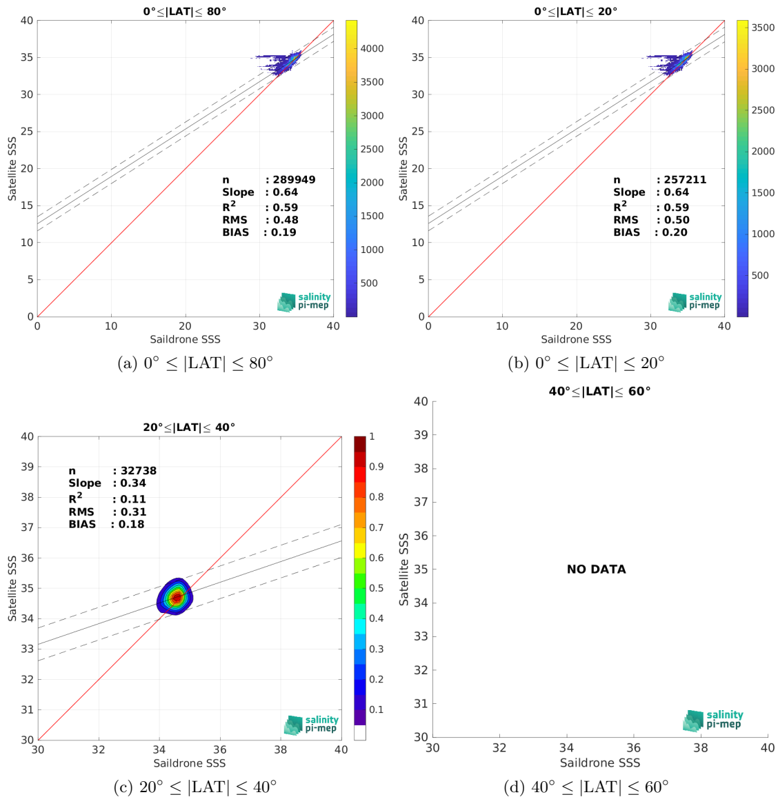
Figure 9: Contour maps of the concentration of SMOS SSS L3 v9 - 9 Days (CATDS-CEC-LOCEAN) SSS (y-axis) versus Saildrone SSS (x-axis) at match-up pairs for different latitude bands. For each plot, the red line shows x=y . The black thin and dashed lines indicate a linear fit through the data cloud and the \pm 95\% confidence levels, respectively. The number match-up pairs n , the slope and R^2 coefficient of the linear fit, the root mean square (RMS) and the mean bias between satellite and in situ data are indicated for each latitude band in each plots.
