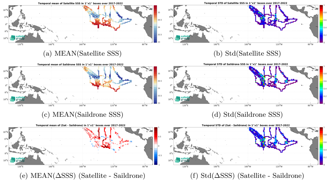
Figure 6: Temporal mean (left) and Std (right) of SSS from SMOS SSS L3 v9 - 9 Days (CATDS-CEC-LOCEAN) (top), Saildrone (middle), and of \Delta SSS (Satellite - Saildrone). Only match-up pairs are used to generate these maps.
