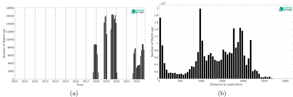
Figure 1: Number of match-ups between Saildrone and SMOS SSS L3 v9 - 9 Days (CATDS-CEC-LOCEAN) SSS as a function of time (a) and as function of the distance to coast (b) over the Tropical Pacific Ocean Pi-MEP region and for the full satellite product period.
