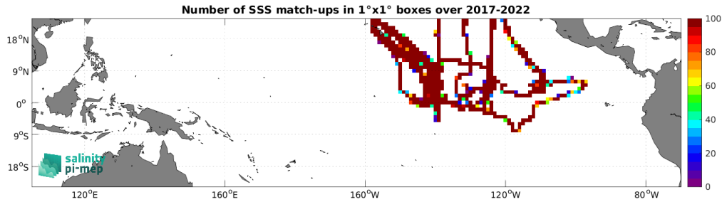
Figure 4: Number of SSS match-ups between Saildrone SSS and the SMOS SSS L3 v9 - 9 Days (CATDS-CEC-LOCEAN) SSS product for the Tropical Pacific Ocean Pi-MEP region over 1^\circ \times 1^\circ boxes and for the full satellite product period.
