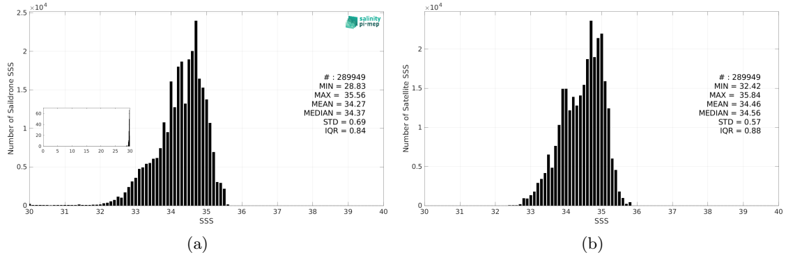
Figure 2: Histograms of SSS from Saildrone (a) and SMOS SSS L3 v9 - 9 Days (CATDS-CEC-LOCEAN) (b) considering all match-up pairs per bins of 0.1 over the Tropical Pacific Ocean Pi-MEP region and for the full satellite product period.
