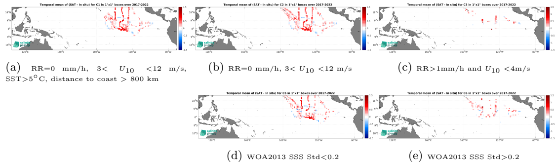
Figure 12: Temporal mean gridded over spatial boxes of size 1^\circ \times 1^\circ of \Delta SSS (SMOS SSS L3 v9 - 9 Days (CATDS-CEC-LOCEAN) - Saldrone) for 5 different subdatasets corresponding to:RR=0 mm/h, 3 < U_{10} < 12 m/s, SST > 5^\circ\text{C} , distance to coast > 800 km (a), RR=0 mm/h, 3 < U_{10} < 12 m/s (b), RR > 1 mm/h and U_{10} < 4 m/s (c), WOA2013 SSS Std < 0.2 (d), WOA2013 SSS Std > 0.2 (e).
