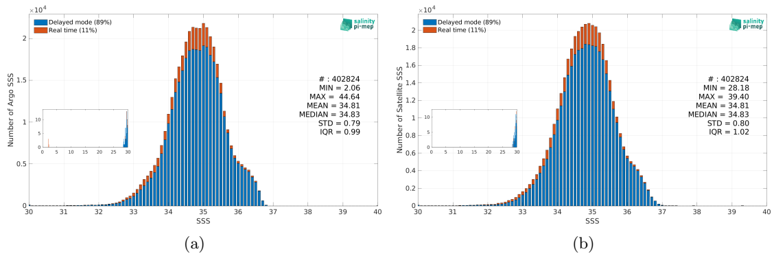
Figure 3: Histograms of SSS from Argo (a) and SMOS SSS L3 v9 - 9 Days (CATDS-CEC-LOCEAN) (b) considering all match-up pairs per bins of 0.1 over the Tropical Pacific Ocean Pi-MEP region and for the full satellite product period.
