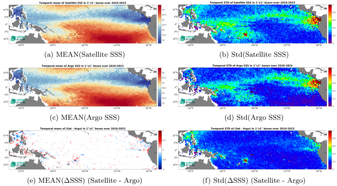
Figure 7: Temporal mean (left) and Std (right) of SSS from SMOS SSS L3 v9 - 9 Days (CATDS-CEC-LOCEAN) (top), Argo (middle), and of \Delta SSS (Satellite - Argo). Only match-up pairs are used to generate these maps.
