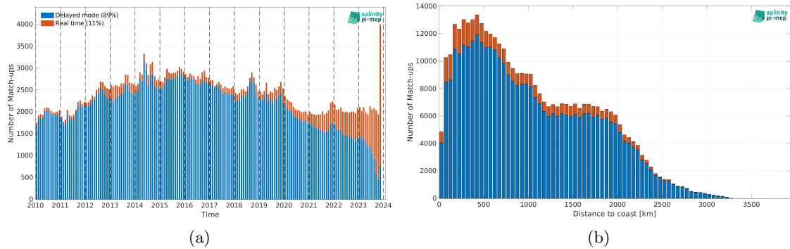
Figure 2: Number of match-ups between Argo and SMOS SSS L3 v9 - 9 Days (CATDS-CEC-LOCEAN) SSS as a function of time (a) and as function of the distance to coast (b) over the Tropical Pacific Ocean Pi-MEP region and for the full satellite product period.
