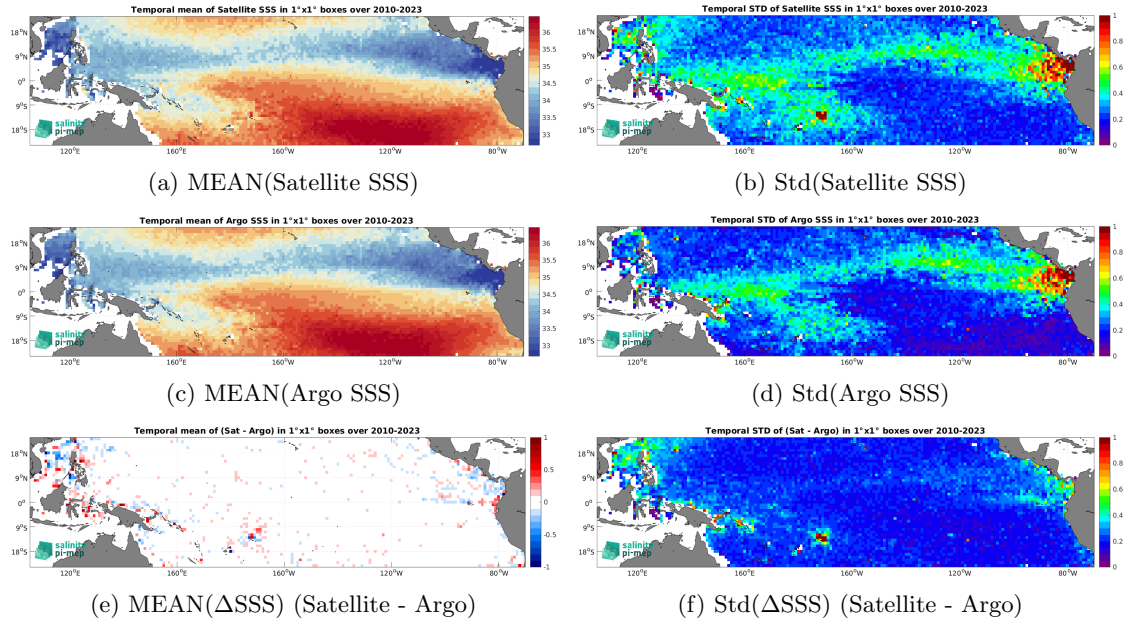
Figure 6: Temporal mean (left) and Std (right) of SSS from SMOS SSS L3 v9 - 9 Days (CATDS-CEC-LOCEAN) (top), Argo (middle), and of \Delta SSS (Satellite - Argo). Only match-up pairs are used to generate these maps.
