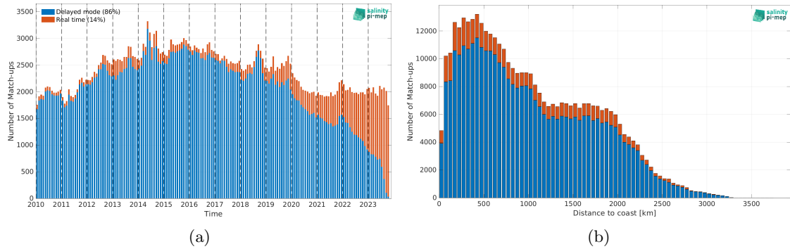
Figure 1: Number of match-ups between Argo and SMOS SSS L3 v9 - 9 Days (CATDS-CEC-LOCEAN) SSS as a function of time (a) and as function of the distance to coast (b) over the Tropical Pacific Ocean Pi-MEP region and for the full satellite product period.
