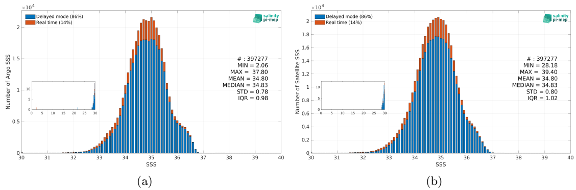
Figure 2: Histograms of SSS from Argo (a) and SMOS SSS L3 v9 - 9 Days (CATDS-CEC-LOCEAN) (b) considering all match-up pairs per bins of 0.1 over the Tropical Pacific Ocean Pi-MEP region and for the full satellite product period.
