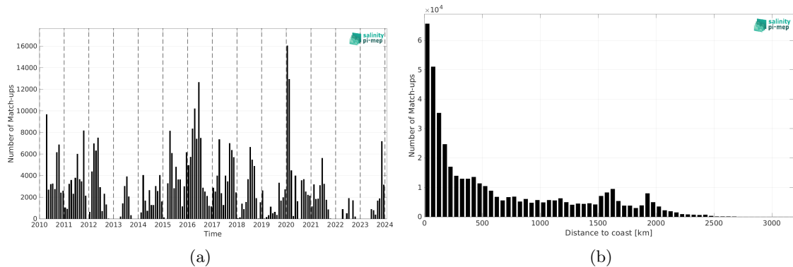
Figure 2: Number of match-ups between TSG (SAMOS) and SMOS SSS L3 v9 - 18 Days (CATDS-CEC-LOCEAN) SSS as a function of time (a) and as function of the distance to coast (b) over the Tropical Pacific Ocean Pi-MEP region and for the full satellite product period.
