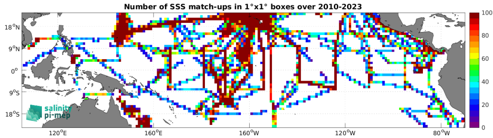
Figure 5: Number of SSS match-ups between TSG (SAMOS) SSS and the SMOS SSS L3 v9 - 18 Days (CATDS-CEC-LOCEAN) SSS product for the Tropical Pacific Ocean Pi-MEP region over 1^\circ \times 1^\circ boxes and for the full satellite product period.
