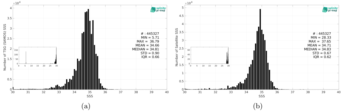
Figure 3: Histograms of SSS from TSG (SAMOS) (a) and SMOS SSS L3 v9 - 18 Days (CATDS-CEC-LOCEAN) (b) considering all match-up pairs per bins of 0.1 over the Tropical Pacific Ocean Pi-MEP region and for the full satellite product period.
