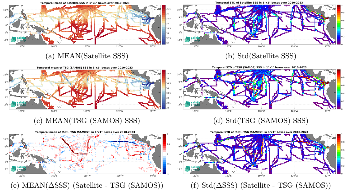
Figure 7: Temporal mean (left) and Std (right) of SSS from SMOS SSS L3 v9 - 18 Days (CATDS-CEC-LOCEAN) (top), TSG (SAMOS) (middle), and of \Delta SSS (Satellite - TSG (SAMOS)). Only match-up pairs are used to generate these maps.
