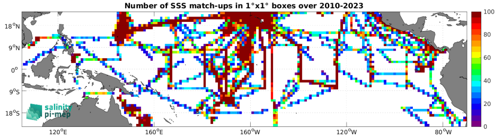
Figure 5: Number of SSS match-ups between TSG (SAMOS) SSS and the SMOS SSS L3 v9 - 18 Days (CATDS-CEC-LOCEAN) SSS product for the Tropical Pacific Ocean Pi-MEP region over 1^\circ \times 1^\circ boxes and for the full satellite product period.
