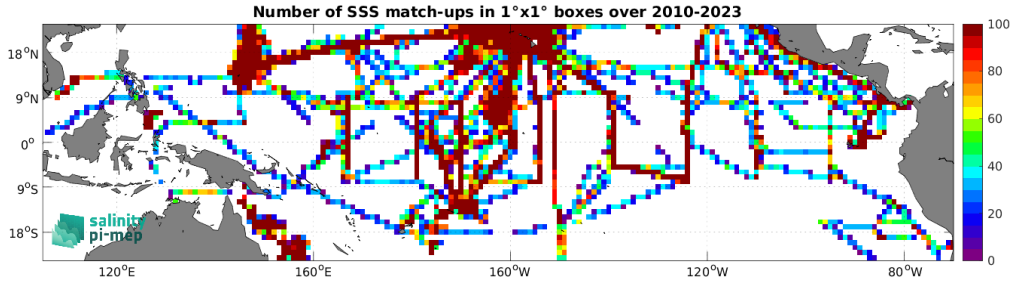
Figure 4: Number of SSS match-ups between TSG (SAMOS) SSS and the SMOS SSS L3 v9 - 18 Days (CATDS-CEC-LOCEAN) SSS product for the Tropical Pacific Ocean Pi-MEP region over 1^\circ \times 1^\circ boxes and for the full satellite product period.
