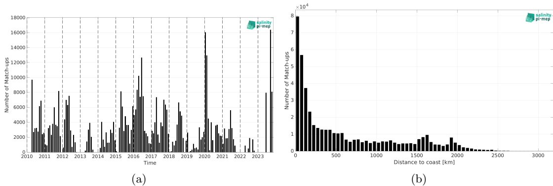
Figure 1: Number of match-ups between TSG (SAMOS) and SMOS SSS L3 v9 - 18 Days (CATDS-CEC-LOCEAN) SSS as a function of time (a) and as function of the distance to coast (b) over the Tropical Pacific Ocean Pi-MEP region and for the full satellite product period.
