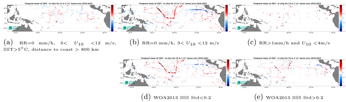
Figure 12: Temporal mean gridded over spatial boxes of size 1^\circ \times 1^\circ of \Delta SSS (SMOS SSS L3 v9 - 18 Days (CATDS-CEC-LOCEAN) - TSG (SAMOS)) for 5 different subdatasets corresponding to: RR=0 mm/h, 3 < U_{10} < 12 m/s, SST > 5^\circ\text{C} , distance to coast > 800 km (a), RR=0 mm/h, 3 < U_{10} < 12 m/s (b), RR > 1 mm/h and U_{10} < 4 m/s (c), WOA2013 SSS Std < 0.2 (d), WOA2013 SSS Std > 0.2 (e).
