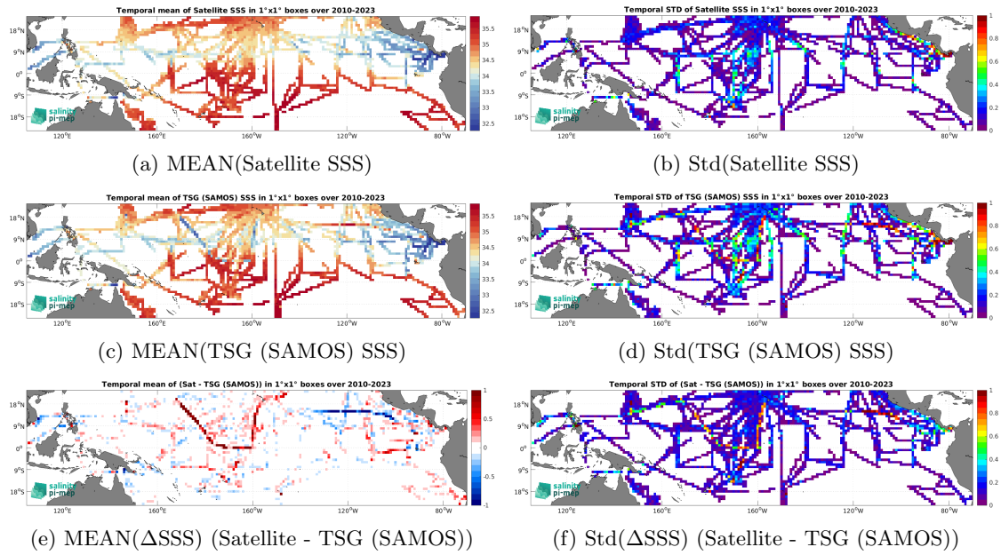
Figure 6: Temporal mean (left) and Std (right) of SSS from SMOS SSS L3 v9 - 18 Days (CATDS-CEC-LOCEAN) (top), TSG (SAMOS) (middle), and of \Delta SSS (Satellite - TSG (SAMOS)). Only match-up pairs are used to generate these maps.
