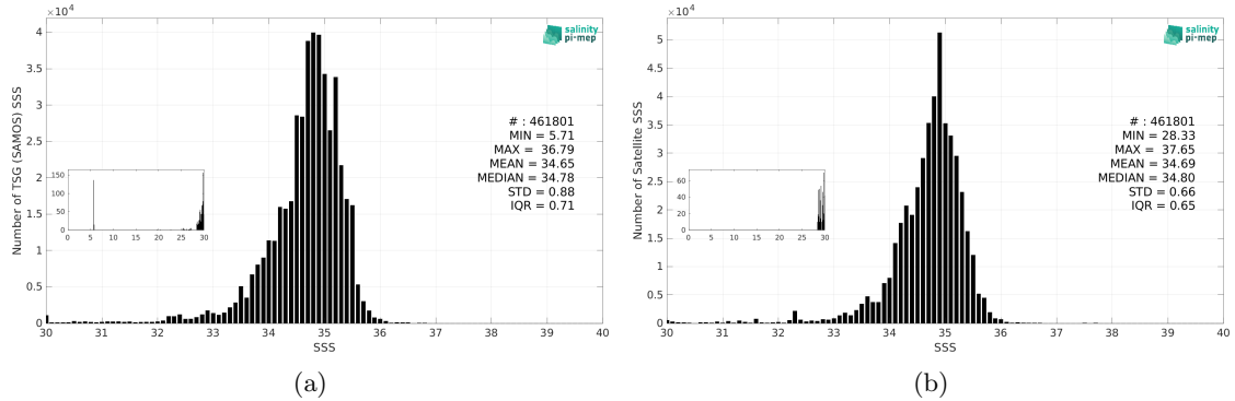
Figure 2: Histograms of SSS from TSG (SAMOS) (a) and SMOS SSS L3 v9 - 18 Days (CATDS-CEC-LOCEAN) (b) considering all match-up pairs per bins of 0.1 over the Tropical Pacific Ocean Pi-MEP region and for the full satellite product period.
