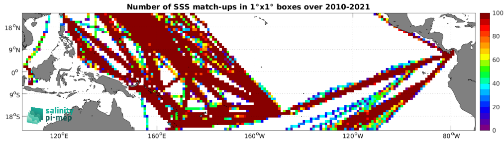
Figure 4: Number of SSS match-ups between TSG (LEGOS-DM) SSS and the SMOS SSS L3 v9 - 18 Days (CATDS-CEC-LOCEAN) SSS product for the Tropical Pacific Ocean Pi-MEP region over 1^\circ \times 1^\circ boxes and for the full satellite product period.
