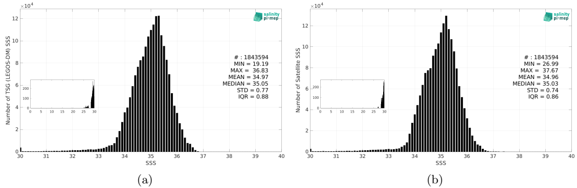
Figure 2: Histograms of SSS from TSG (LEGOS-DM) (a) and SMOS SSS L3 v9 - 18 Days (CATDS-CEC-LOCEAN) (b) considering all match-up pairs per bins of 0.1 over the Tropical Pacific Ocean Pi-MEP region and for the full satellite product period.
