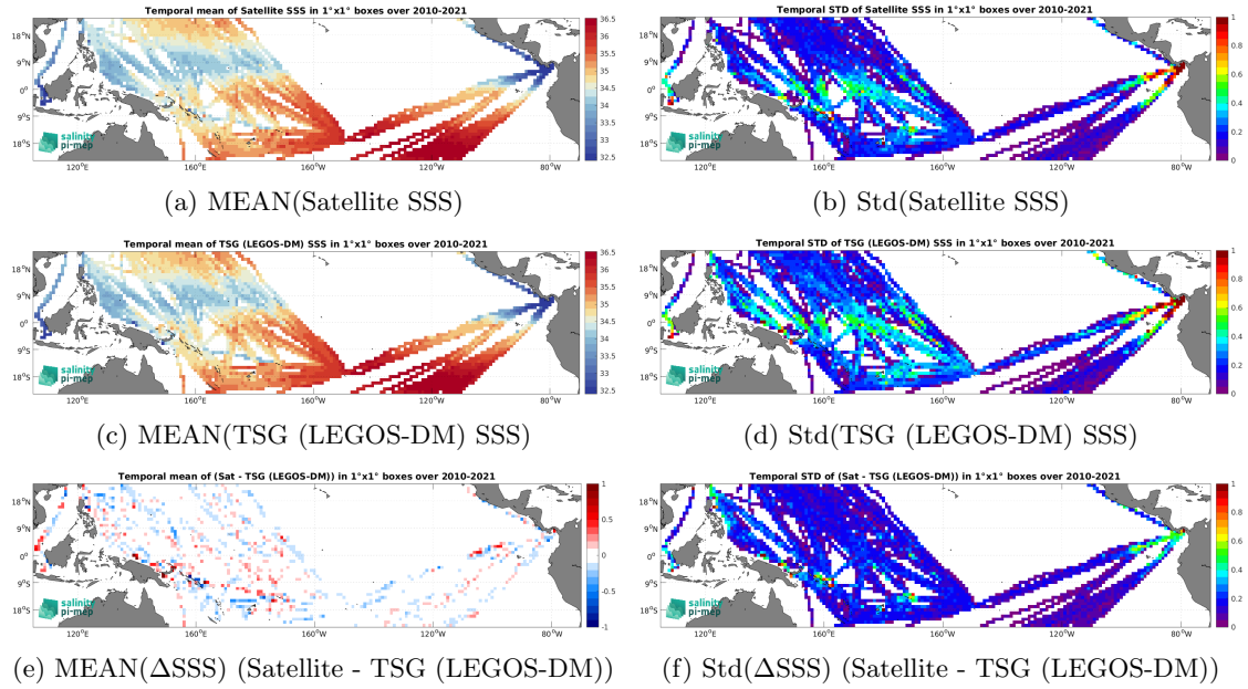
Figure 6: Temporal mean (left) and Std (right) of SSS from SMOS SSS L3 v9 - 18 Days (CATDS-CEC-LOCEAN) (top), TSG (LEGOS-DM) (middle), and of \Delta SSS (Satellite - TSG (LEGOS-DM)). Only match-up pairs are used to generate these maps.
