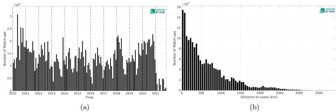
Figure 1: Number of match-ups between TSG (LEGOS-DM) and SMOS SSS L3 v9 - 18 Days (CATDS-CEC-LOCEAN) SSS as a function of time (a) and as function of the distance to coast (b) over the Tropical Pacific Ocean Pi-MEP region and for the full satellite product period.
