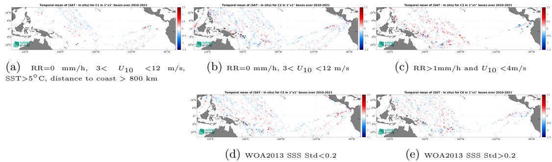
Figure 12: Temporal mean gridded over spatial boxes of size 1^{\circ}\times 1^{\circ} of \Delta\text{SSS} (SMOS SSS L3 v9 - 18 Days (CATDS-CEC-LOCEAN) - TSG (LEGOS-DM)) for 5 different subdatasets corresponding to:RR=0 mm/h, 3 < U_{10} < 12 m/s, SST > 5^{\circ}\text{C} , distance to coast > 800 km (a), RR=0 mm/h, 3 < U_{10} < 12 m/s (b), RR > 1 mm/h and U_{10} < 4 m/s (c), WOA2013 SSS Std < 0.2 (d), WOA2013 SSS Std > 0.2 (e).
