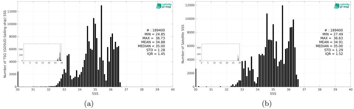
Figure 3: Histograms of SSS from TSG (GOSUD-Sailing-ship) (a) and SMOS SSS L3 v9 - 18 Days (CATDS-CEC-LOCEAN) (b) considering all match-up pairs per bins of 0.1 over the Tropical Pacific Ocean Pi-MEP region and for the full satellite product period.
