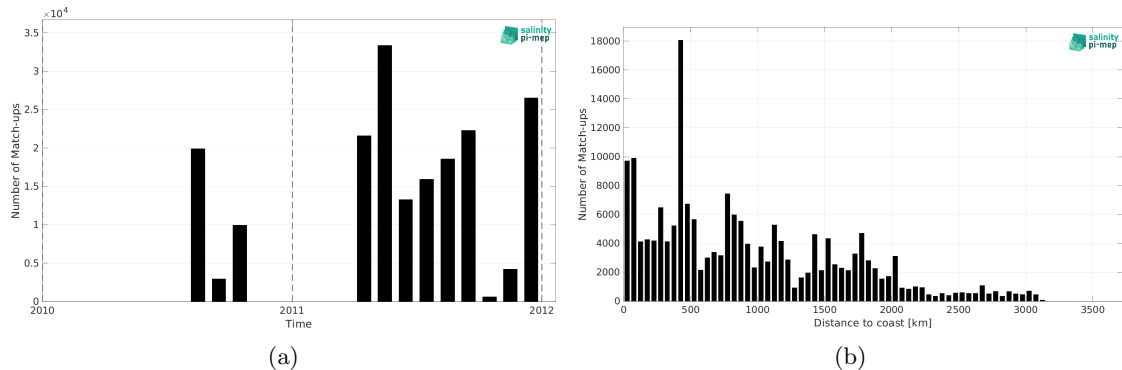
Figure 2: Number of match-ups between TSG (GOSUD-Sailing-ship) and SMOS SSS L3 v9 - 18 Days (CATDS-CEC-LOCEAN) SSS as a function of time (a) and as function of the distance to coast (b) over the Tropical Pacific Ocean Pi-MEP region and for the full satellite product period.
