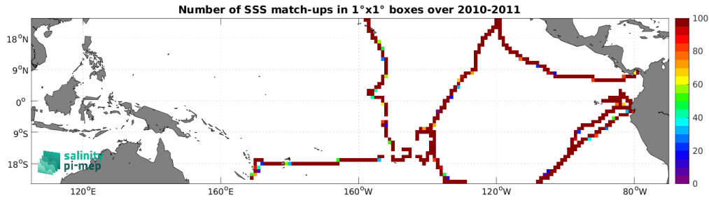
Figure 4: Number of SSS match-ups between TSG (GOSUD-Sailing-ship) SSS and the SMOS SSS L3 v9 - 18 Days (CATDS-CEC-LOCEAN) SSS product for the Tropical Pacific Ocean Pi-MEP region over 1^\circ \times 1^\circ boxes and for the full satellite product period.
