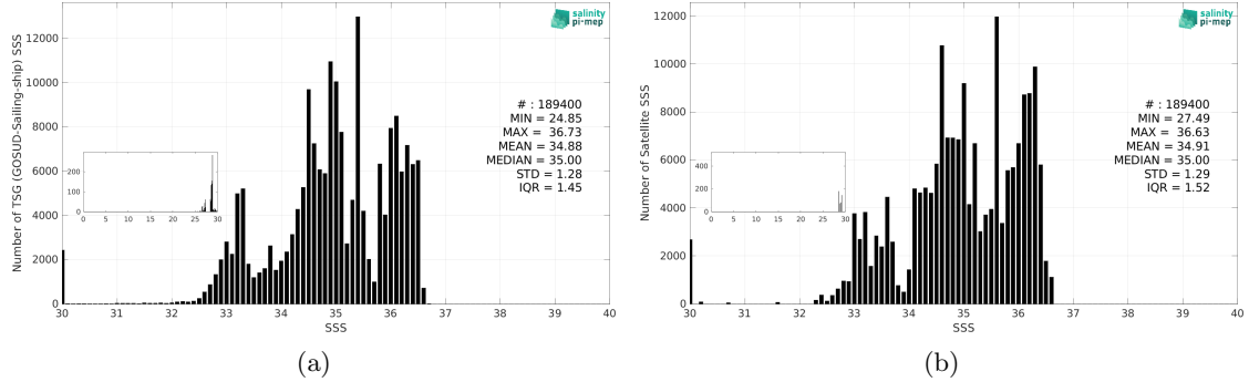
Figure 2: Histograms of SSS from TSG (GOSUD-Sailing-ship) (a) and SMOS SSS L3 v9 - 18 Days (CATDS-CEC-LOCEAN) (b) considering all match-up pairs per bins of 0.1 over the Tropical Pacific Ocean Pi-MEP region and for the full satellite product period.
