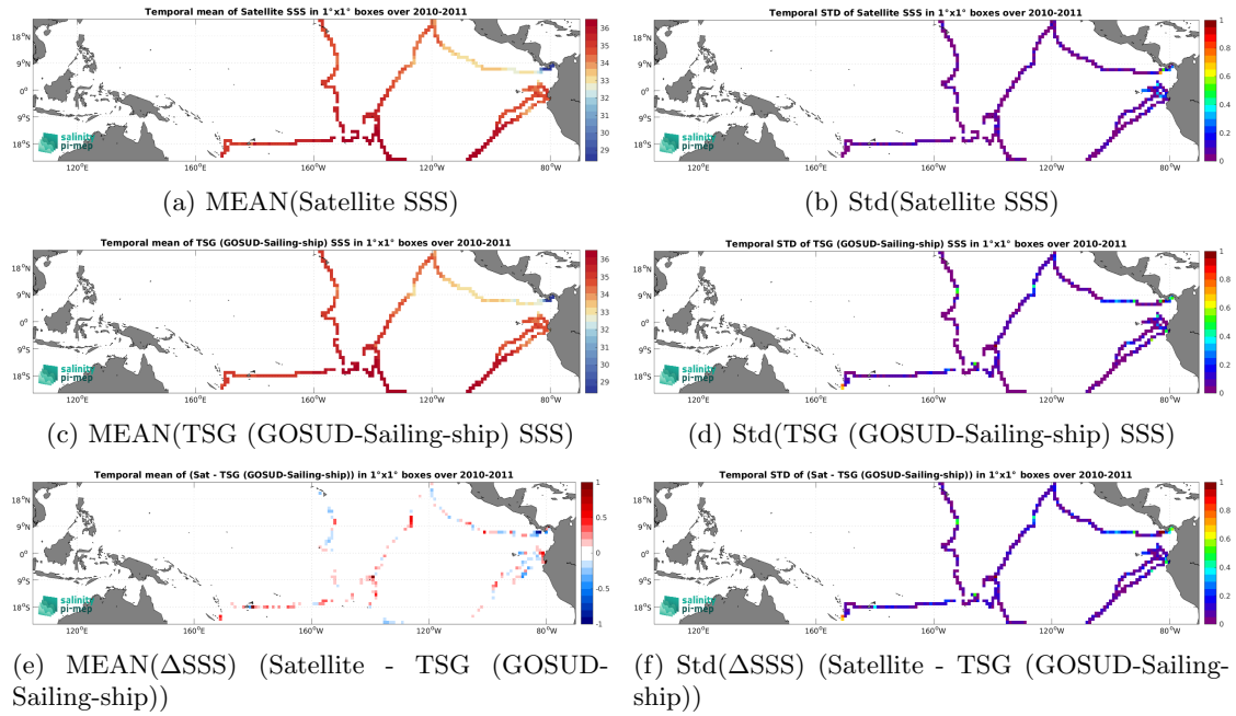
Figure 6: Temporal mean (left) and Std (right) of SSS from SMOS SSS L3 v9 - 18 Days (CATDS-CEC-LOCEAN) (top), TSG (GOSUD-Sailing-ship) (middle), and of \Delta SSS (Satellite - TSG (GOSUD-Sailing-ship)). Only match-up pairs are used to generate these maps.
