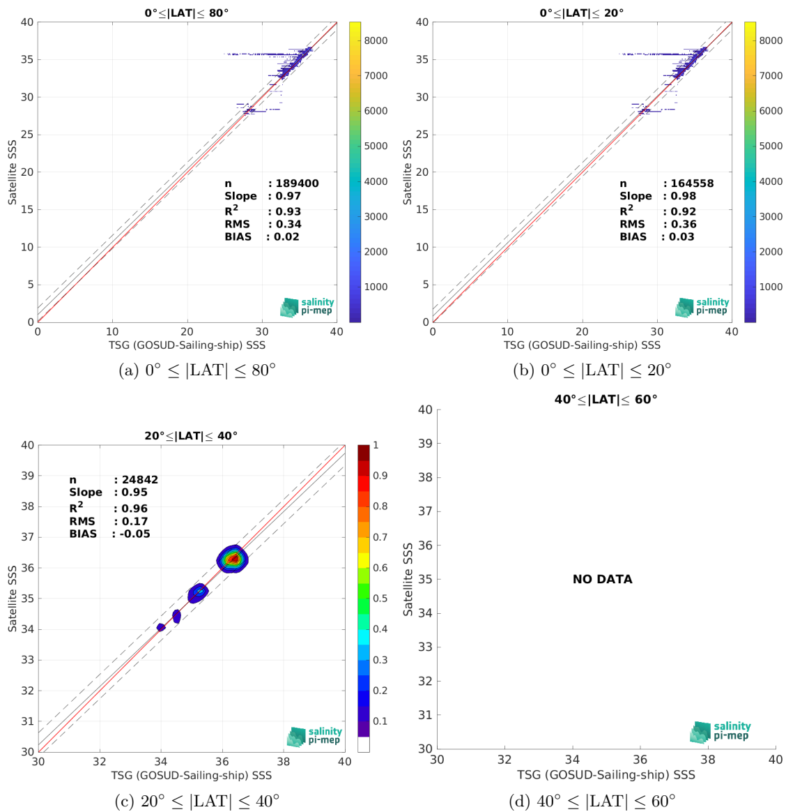
Figure 9: Contour maps of the concentration of SMOS SSS L3 v9 - 18 Days (CATDS-CEC-LOCEAN) SSS (y-axis) versus TSG (GOSUD-Sailing-ship) SSS (x-axis) at match-up pairs for different latitude bands. For each plot, the red line shows x=y . The black thin and dashed lines indicate a linear fit through the data cloud and the \pm 95\% confidence levels, respectively. The number match-up pairs n , the slope and R^2 coefficient of the linear fit, the root mean square (RMS) and the mean bias between satellite and in situ data are indicated for each latitude band in each plots.
