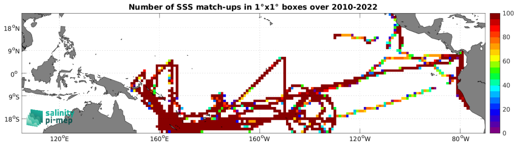
Figure 5: Number of SSS match-ups between TSG (GOSUD-Research-vessel) SSS and the SMOS SSS L3 v9 - 18 Days (CATDS-CEC-LOCEAN) SSS product for the Tropical Pacific Ocean Pi-MEP region over 1^\circ \times 1^\circ boxes and for the full satellite product period.
