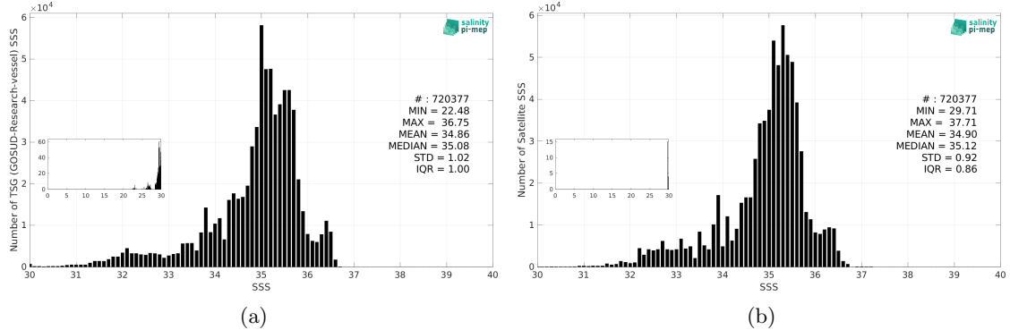
Figure 3: Histograms of SSS from TSG (GOSUD-Research-vessel) (a) and SMOS SSS L3 v9 - 18 Days (CATDS-CEC-LOCEAN) (b) considering all match-up pairs per bins of 0.1 over the Tropical Pacific Ocean Pi-MEP region and for the full satellite product period.
