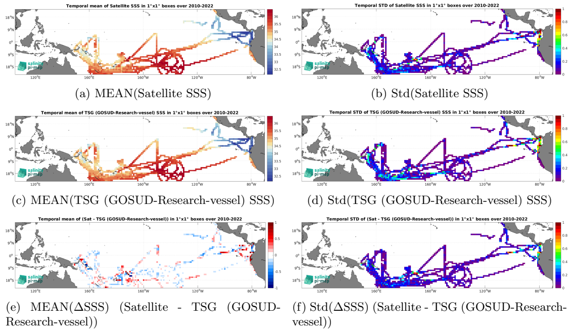
Figure 7: Temporal mean (left) and Std (right) of SSS from SMOS SSS L3 v9 - 18 Days (CATDS-CEC-LOCEAN) (top), TSG (GOSUD-Research-vessel) (middle), and of \Delta SSS (Satellite - TSG (GOSUD-Research-vessel)). Only match-up pairs are used to generate these maps.
