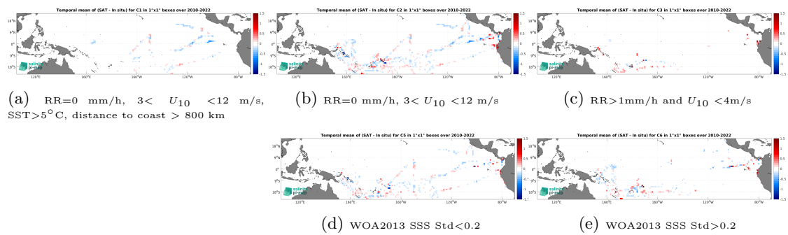
Figure 14: Temporal mean gridded over spatial boxes of size 1^\circ \times 1^\circ of \Delta\text{SSS} (SMOS SSS L3 v9 - 18 Days (CATDS-CEC-LOCEAN) - TSG (GOSUD-Research-vessel)) for 5 different subdatasets corresponding to:RR=0 mm/h, 3 < U_{10} < 12 m/s, SST>5°C, distance to coast > 800 km (a), RR=0 mm/h, 3 < U_{10} < 12 m/s (b), RR>1mm/h and U_{10} < 4 m/s (c), WOA2013 SSS Std<0.2 (d), WOA2013 SSS Std>0.2 (e).
