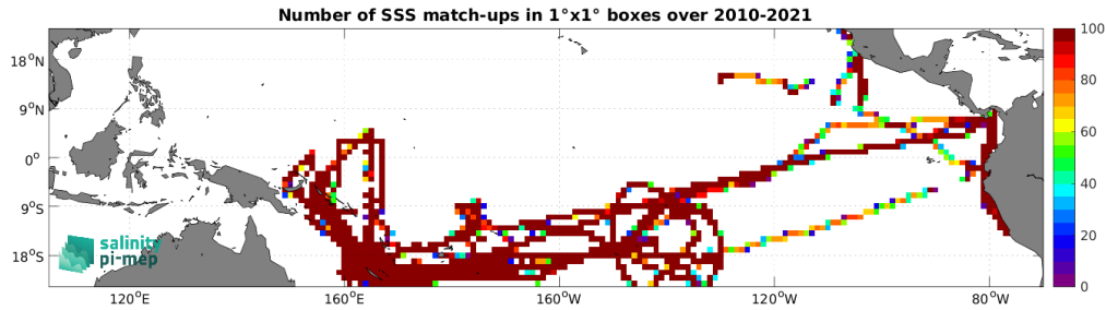
Figure 4: Number of SSS match-ups between TSG (GOSUD-Research-vessel) SSS and the SMOS SSS L3 v9 - 18 Days (CATDS-CEC-LOCEAN) SSS product for the Tropical Pacific Ocean Pi-MEP region over 1^\circ \times 1^\circ boxes and for the full satellite product period.
