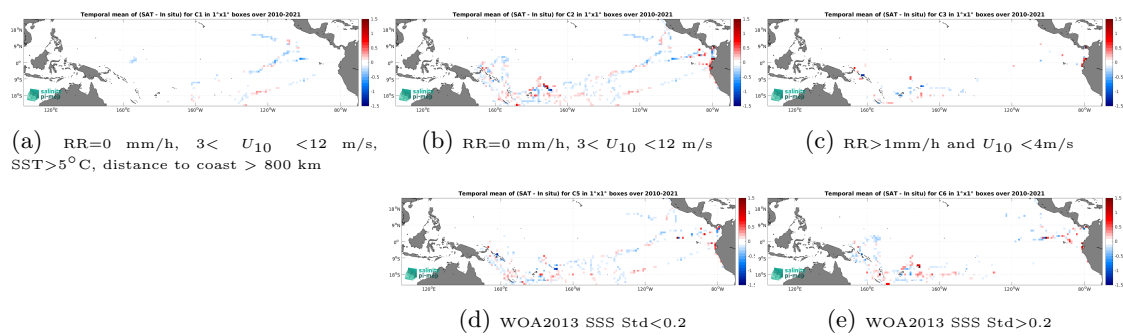
Figure 12: Temporal mean gridded over spatial boxes of size 1^\circ \times 1^\circ of \Delta\text{SSS} (SMOS SSS L3 v9 - 18 Days (CATDS-CEC-LOCEAN) - TSG (GOSUD-Research-vessel)) for 5 different subdatasets corresponding to:RR=0 mm/h, 3 < U_{10} < 12 m/s, SST >5^\circ\text{C} , distance to coast > 800 km (a), RR=0 mm/h, 3 < U_{10} < 12 m/s (b), RR >1 mm/h and U_{10} < 4 m/s (c), WOA2013 SSS Std <0.2 (d), WOA2013 SSS Std >0.2 (e).
