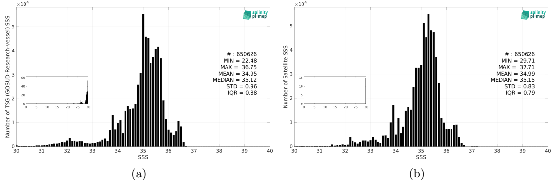
Figure 2: Histograms of SSS from TSG (GOSUD-Research-vessel) (a) and SMOS SSS L3 v9 - 18 Days (CATDS-CEC-LOCEAN) (b) considering all match-up pairs per bins of 0.1 over the Tropical Pacific Ocean Pi-MEP region and for the full satellite product period.
