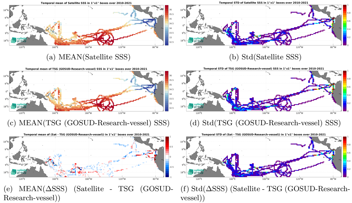
Figure 6: Temporal mean (left) and Std (right) of SSS from SMOS SSS L3 v9 - 18 Days (CATDS-CEC-LOCEAN) (top), TSG (GOSUD-Research-vessel) (middle), and of \Delta SSS (Satellite - TSG (GOSUD-Research-vessel)). Only match-up pairs are used to generate these maps.
