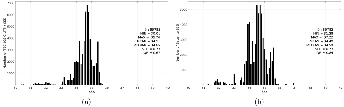
Figure 3: Histograms of SSS from TSG (CSIC-UTM) (a) and SMOS SSS L3 v9 - 18 Days (CATDS-CEC-LOCEAN) (b) considering all match-up pairs per bins of 0.1 over the Tropical Pacific Ocean Pi-MEP region and for the full satellite product period.
