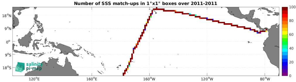
Figure 5: Number of SSS match-ups between TSG (CSIC-UTM) SSS and the SMOS SSS L3 v9 - 18 Days (CATDS-CEC-LOCEAN) SSS product for the Tropical Pacific Ocean Pi-MEP region over 1^\circ \times 1^\circ boxes and for the full satellite product period.
