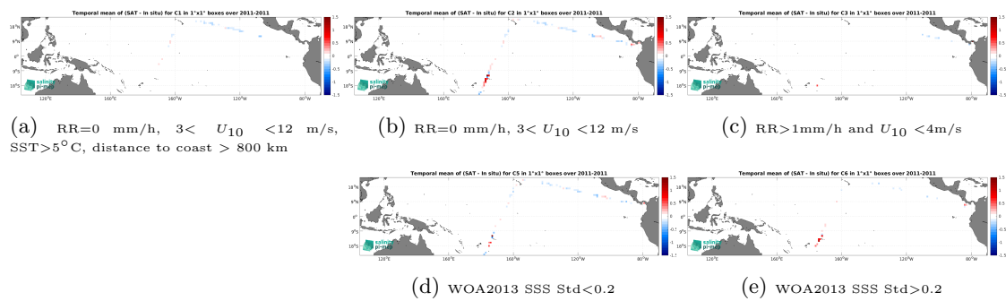
Figure 14: Temporal mean gridded over spatial boxes of size 1^\circ \times 1^\circ of \Delta SSS (SMOS SSS L3 v9 - 18 Days (CATDS-CEC-LOCEAN) - TSG (CSIC-UTM)) for 5 different subdatasets corresponding to:RR=0 mm/h, 3 < U_{10} < 12 m/s, SST > 5^\circ\text{C} , distance to coast > 800 km (a), RR=0 mm/h, 3 < U_{10} < 12 m/s (b), RR > 1 mm/h and U_{10} < 4 m/s (c), WOA2013 SSS Std < 0.2 (d), WOA2013 SSS Std > 0.2 (e).
