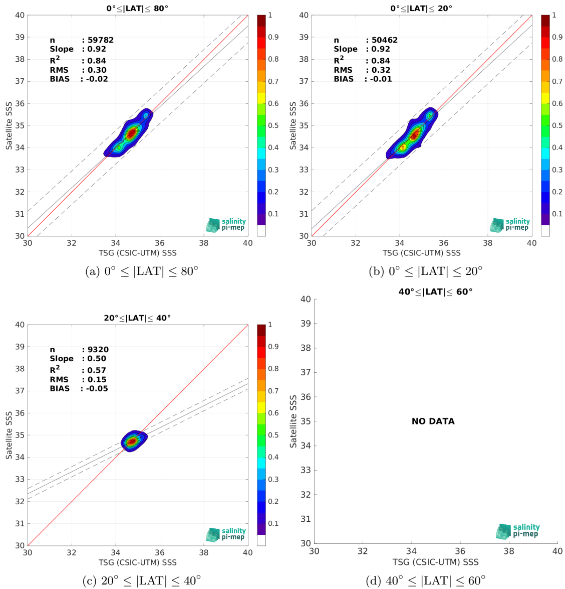
Figure 9: Contour maps of the concentration of SMOS SSS L3 v9 - 18 Days (CATDS-CEC-LOCEAN) SSS (y-axis) versus TSG (CSIC-UTM) SSS (x-axis) at match-up pairs for different latitude bands. For each plot, the red line shows x=y . The black thin and dashed lines indicate a linear fit through the data cloud and the \pm 95\% confidence levels, respectively. The number match-up pairs n , the slope and R^2 coefficient of the linear fit, the root mean square (RMS) and the mean bias between satellite and in situ data are indicated for each latitude band in each plots.
