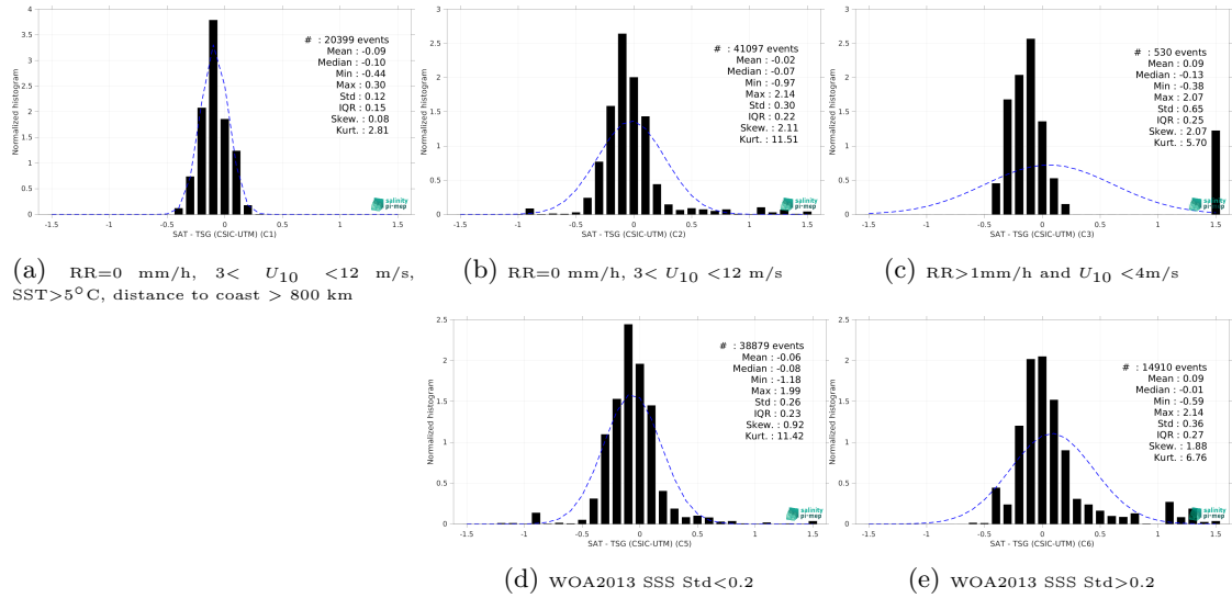
Figure 13: Normalized histogram of \Delta SSS (SMOS SSS L3 v9 - 18 Days (CATDS-CEC-LOCEAN) - TSG (CSIC-UTM)) for 5 different subdatasets corresponding to: RR=0 mm/h, 3 < U_{10} < 12 m/s, SST>5°C, distance to coast > 800 km (a), RR=0 mm/h, 3 < U_{10} < 12 m/s (b), RR>1mm/h and U_{10} < 4 m/s (c), WOA2013 SSS Std<0.2 (d), WOA2013 SSS Std>0.2 (e).
