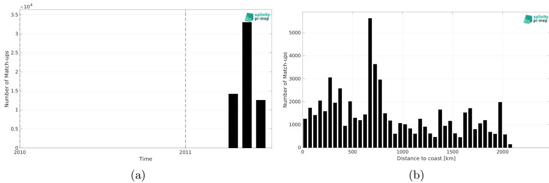
Figure 1: Number of match-ups between TSG (CSIC-UTM) and SMOS SSS L3 v9 - 18 Days (CATDS-CEC-LOCEAN) SSS as a function of time (a) and as function of the distance to coast (b) over the Tropical Pacific Ocean Pi-MEP region and for the full satellite product period.
