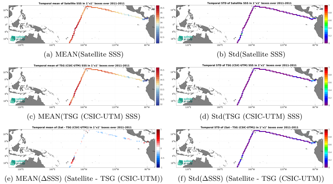
Figure 6: Temporal mean (left) and Std (right) of SSS from SMOS SSS L3 v9 - 18 Days (CATDS-CEC-LOCEAN) (top), TSG (CSIC-UTM) (middle), and of \Delta SSS (Satellite - TSG (CSIC-UTM)). Only match-up pairs are used to generate these maps.
