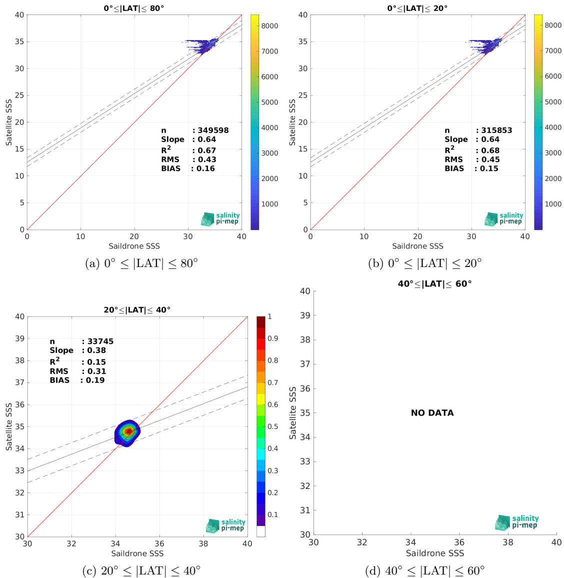
Figure 10: Contour maps of the concentration of SMOS SSS L3 v9 - 18 Days (CATDS-CEC-LOCEAN) SSS (y-axis) versus Sairdrone SSS (x-axis) at match-up pairs for different latitude bands. For each plot, the red line shows x=y . The black thin and dashed lines indicate a linear fit through the data cloud and the \pm 95\% confidence levels, respectively. The number match-up pairs n , the slope and R^2 coefficient of the linear fit, the root mean square (RMS) and the mean bias between satellite and in situ data are indicated for each latitude band in each plots.
