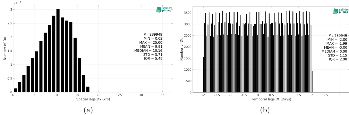
Figure 6: Histograms of the spatial (a) and temporal (b) lags between the location/time of the Sairdrone measurement and the date of the corresponding SMOS SSS L3 v9 - 18 Days (CATDS-CEC-LOCEAN) SSS pixel.
