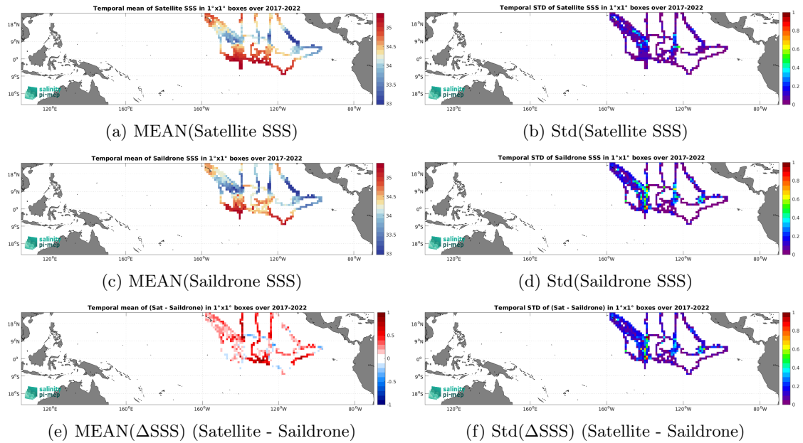
Figure 7: Temporal mean (left) and Std (right) of SSS from SMOS SSS L3 v9 - 18 Days (CATDS-CEC-LOCEAN) (top), Saildrone (middle), and of \Delta SSS (Satellite - Saildrone). Only match-up pairs are used to generate these maps.
