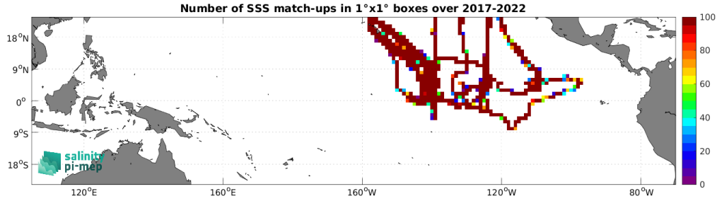
Figure 5: Number of SSS match-ups between Sairdrone SSS and the SMOS SSS L3 v9 - 18 Days (CATDS-CEC-LOCEAN) SSS product for the Tropical Pacific Ocean Pi-MEP region over 1^\circ \times 1^\circ boxes and for the full satellite product period.
