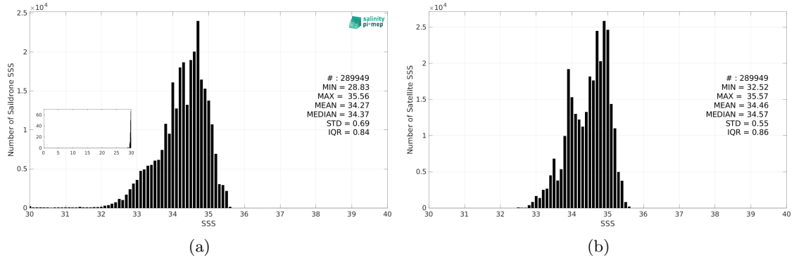
Figure 3: Histograms of SSS from Saildrone (a) and SMOS SSS L3 v9 - 18 Days (CATDS-CEC-LOCEAN) (b) considering all match-up pairs per bins of 0.1 over the Tropical Pacific Ocean Pi-MEP region and for the full satellite product period.
