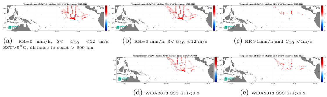
Figure 14: Temporal mean gridded over spatial boxes of size 1^\circ \times 1^\circ of \Delta SSS (SMOS SSS L3 v9 - 18 Days (CATDS-CEC-LOCEAN) - Saildrone) for 5 different subdatasets corresponding to: RR=0 mm/h, 3 < U_{10} < 12 m/s, SST > 5°C, distance to coast > 800 km (a), RR=0 mm/h, 3 < U_{10} < 12 m/s (b), RR > 1mm/h and U_{10} < 4 m/s (c), WOA2013 SSS Std < 0.2 (d), WOA2013 SSS Std > 0.2 (e).
