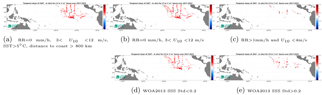
Figure 12: Temporal mean gridded over spatial boxes of size 1^\circ \times 1^\circ of \Delta SSS (SMOS SSS L3 v9 - 18 Days (CATDS-CEC-LOCEAN) - Sairdrone) for 5 different subdatasets corresponding to: RR=0 mm/h, 3 < U_{10} < 12 m/s, SST > 5^\circ\text{C} , distance to coast > 800 km (a), RR=0 mm/h, 3 < U_{10} < 12 m/s (b), RR > 1 mm/h and U_{10} < 4 m/s (c), WOA2013 SSS Std < 0.2 (d), WOA2013 SSS Std > 0.2 (e).
