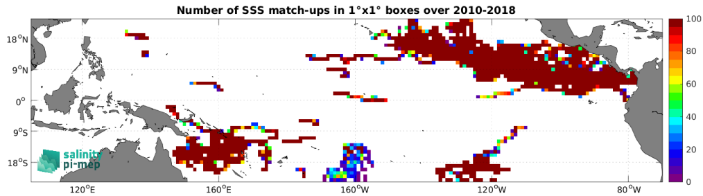
Figure 3: Number of SSS match-ups between Surface drifters SSS and the SMOS SSS L3 v9 - 18 Days (CATDS-CEC-LOCEAN) SSS product for the Tropical Pacific Ocean Pi-MEP region over 1^\circ \times 1^\circ boxes and for the full satellite product period.
