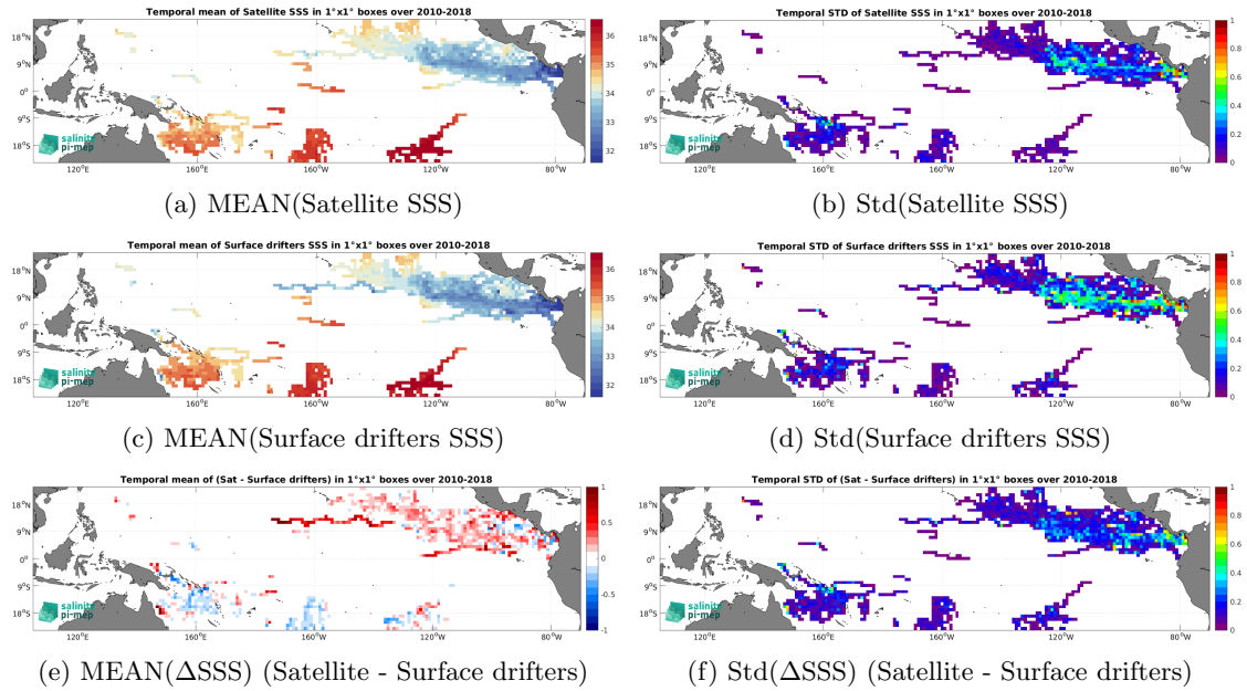
Figure 5: Temporal mean (left) and Std (right) of SSS from SMOS SSS L3 v9 - 18 Days (CATDS-CEC-LOCEAN) (top), Surface drifters (middle), and of \Delta SSS (Satellite - Surface drifters). Only match-up pairs are used to generate these maps.
