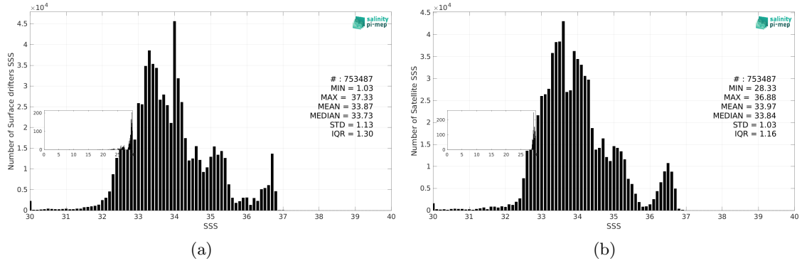
Figure 2: Histograms of SSS from Surface drifters (a) and SMOS SSS L3 v9 - 18 Days (CATDS-CEC-LOCEAN) (b) considering all match-up pairs per bins of 0.1 over the Tropical Pacific Ocean Pi-MEP region and for the full satellite product period.
