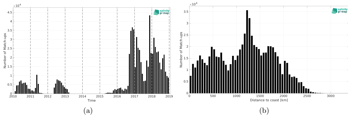
Figure 1: Number of match-ups between Surface drifters and SMOS SSS L3 v9 - 18 Days (CATDS-CEC-LOCEAN) SSS as a function of time (a) and as function of the distance to coast (b) over the Tropical Pacific Ocean Pi-MEP region and for the full satellite product period.
