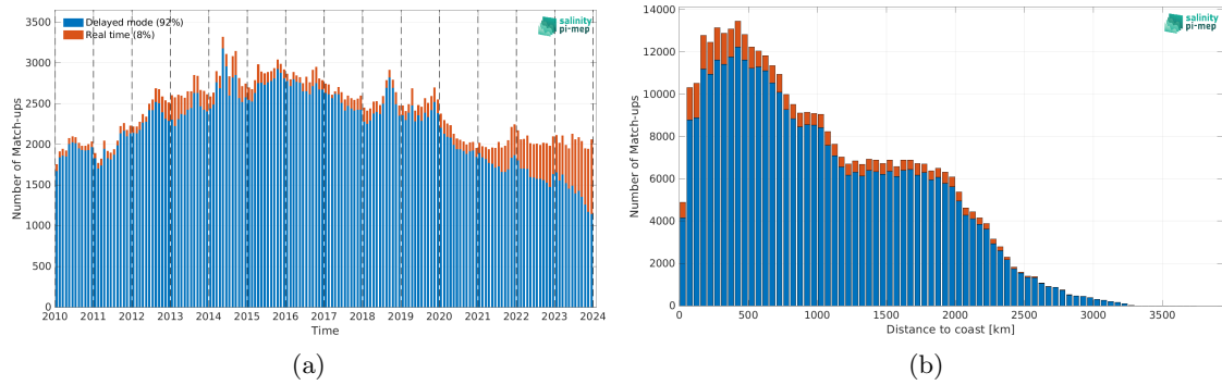
Figure 2: Number of match-ups between Argo and SMOS SSS L3 v9 - 18 Days (CATDS-CEC-LOCEAN) SSS as a function of time (a) and as function of the distance to the coast (b) over the Tropical Pacific Ocean Pi-MEP region and for the full satellite product period.
