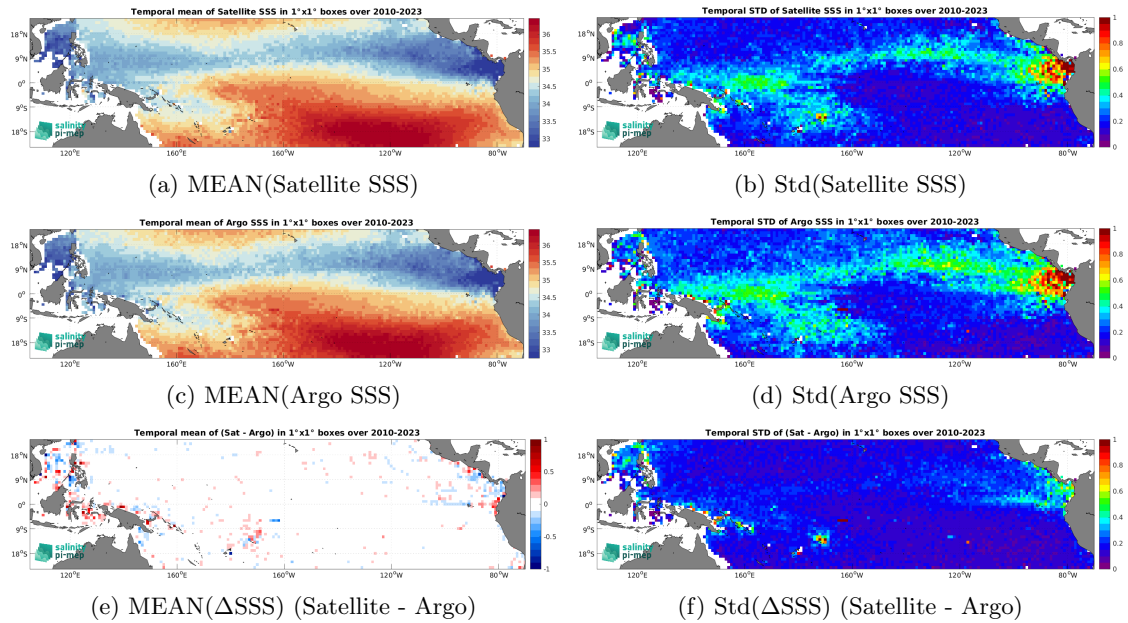
Figure 7: Temporal mean (left) and Std (right) of SSS from SMOS SSS L3 v9 - 18 Days (CATDS-CEC-LOCEAN) (top), Argo (middle), and of \Delta SSS (Satellite - Argo). Only match-up pairs are used to generate these maps.
