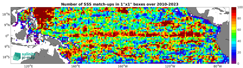
Figure 5: Number of SSS match-ups between Argo SSS and the SMOS SSS L3 v9 - 18 Days (CATDS-CEC-LOCEAN) SSS product for the Tropical Pacific Ocean Pi-MEP region over 1^\circ \times 1^\circ boxes and for the full satellite product period.
