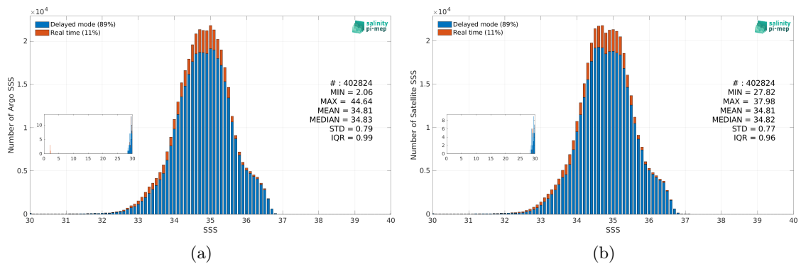
Figure 3: Histograms of SSS from Argo (a) and SMOS SSS L3 v9 - 18 Days (CATDS-CEC-LOCEAN) (b) considering all match-up pairs per bins of 0.1 over the Tropical Pacific Ocean Pi-MEP region and for the full satellite product period.
