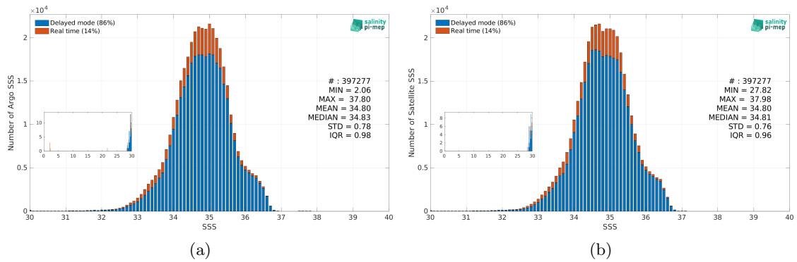
Figure 2: Histograms of SSS from Argo (a) and SMOS SSS L3 v9 - 18 Days (CATDS-CEC-LOCEAN) (b) considering all match-up pairs per bins of 0.1 over the Tropical Pacific Ocean Pi-MEP region and for the full satellite product period.
