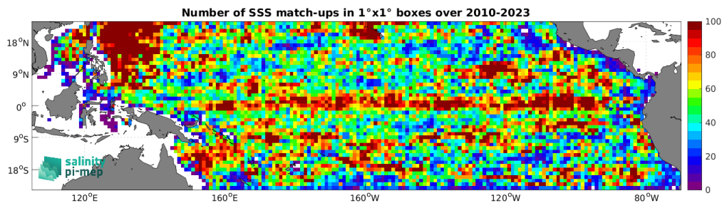
Figure 4: Number of SSS match-ups between Argo SSS and the SMOS SSS L3 v9 - 18 Days (CATDS-CEC-LOCEAN) SSS product for the Tropical Pacific Ocean Pi-MEP region over 1^\circ \times 1^\circ boxes and for the full satellite product period.
