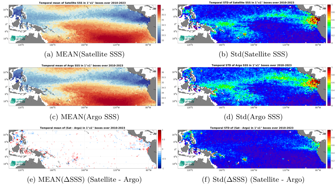
Figure 6: Temporal mean (left) and Std (right) of SSS from SMOS SSS L3 v9 - 18 Days (CATDS-CEC-LOCEAN) (top), Argo (middle), and of \Delta SSS (Satellite - Argo). Only match-up pairs are used to generate these maps.
