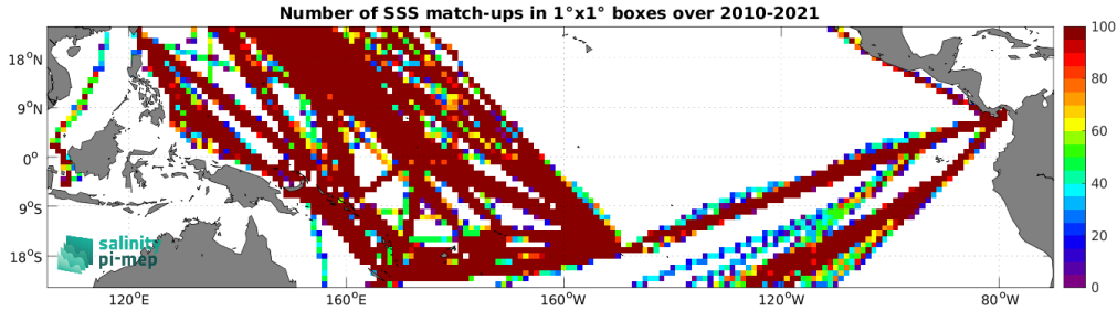
Figure 4: Number of SSS match-ups between TSG (LEGOS-DM) SSS and the SMOS SSS L3 v8 - 9 Days (CATDS-CEC-LOCEAN) SSS product for the Tropical Pacific Ocean Pi-MEP region over 1^\circ \times 1^\circ boxes and for the full satellite product period.
