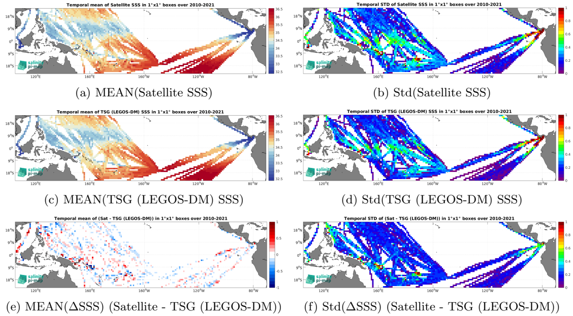
Figure 6: Temporal mean (left) and Std (right) of SSS from SMOS SSS L3 v8 - 9 Days (CATDS-CEC-LOCEAN) (top), TSG (LEGOS-DM) (middle), and of \Delta SSS (Satellite - TSG (LEGOS-DM)). Only match-up pairs are used to generate these maps.
