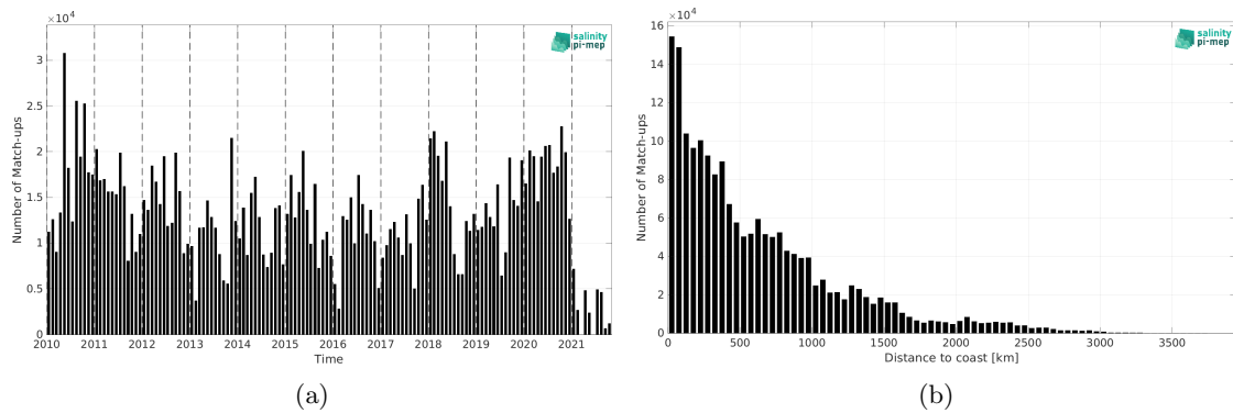
Figure 1: Number of match-ups between TSG (LEGOS-DM) and SMOS SSS L3 v8 - 9 Days (CATDS-CEC-LOCEAN) SSS as a function of time (a) and as function of the distance to coast (b) over the Tropical Pacific Ocean Pi-MEP region and for the full satellite product period.
