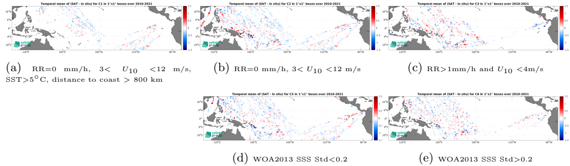
Figure 12: Temporal mean gridded over spatial boxes of size 1^{\circ}\times 1^{\circ} of \Delta\text{SSS} (SMOS SSS L3 v8 - 9 Days (CATDS-CEC-LOCEAN) - TSG (LEGOS-DM)) for 5 different subdatasets corresponding to:RR=0 mm/h, 3 < U_{10} < 12 m/s, SST >5^{\circ}\text{C} , distance to coast > 800 km (a), RR=0 mm/h, 3 < U_{10} < 12 m/s (b), RR >1 mm/h and U_{10} < 4 m/s (c), WOA2013 SSS Std <0.2 (d), WOA2013 SSS Std >0.2 (e).
