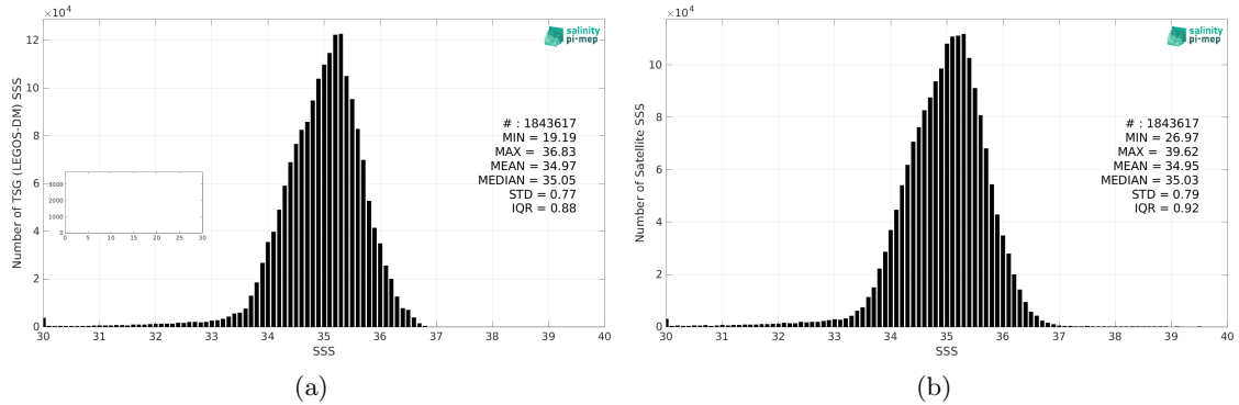
Figure 2: Histograms of SSS from TSG (LEGOS-DM) (a) and SMOS SSS L3 v8 - 9 Days (CATDS-CEC-LOCEAN) (b) considering all match-up pairs per bins of 0.1 over the Tropical Pacific Ocean Pi-MEP region and for the full satellite product period.
