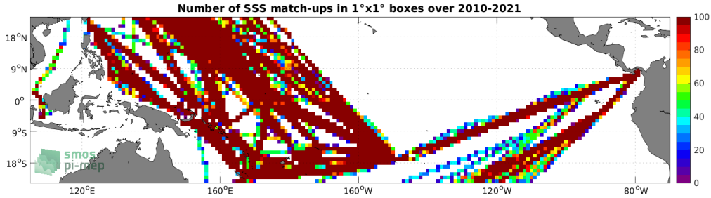
Figure 4: Number of SSS match-ups between TSG (LEGOS-DM) SSS and the SMOS SSS L3 v8 - 9 Days (CATDS-CECOS-LOCEAN) SSS product for the Tropical Pacific Ocean Pi-MEP region over 1^\circ \times 1^\circ boxes and for the full satellite product period.
