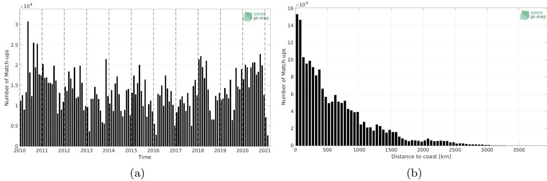
Figure 1: Number of match-ups between TSG (LEGOS-DM) and SMOS SSS L3 v8 - 9 Days (CATDS-CECOS-LOCEAN) SSS as a function of time (a) and as function of the distance to coast (b) over the Tropical Pacific Ocean Pi-MEP region and for the full satellite product period.
