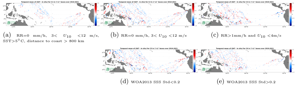
Figure 12: Temporal mean gridded over spatial boxes of size 1^{\circ}\times 1^{\circ} of \Delta\text{SSS} (SMOS SSS L3 v8 - 9 Days (CATDS-CECOS-LOCEAN) - TSG (LEGOS-DM)) for 5 different subdatasets corresponding to:RR=0 mm/h, 3 < U_{10} < 12 m/s, SST > 5^{\circ}\text{C} , distance to coast > 800 km (a), RR=0 mm/h, 3 < U_{10} < 12 m/s (b), RR > 1 mm/h and U_{10} < 4 m/s (c), WOA2013 SSS Std < 0.2 (d), WOA2013 SSS Std > 0.2 (e).
