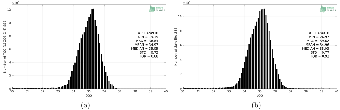
Figure 2: Histograms of SSS from TSG (LEGOS-DM) (a) and SMOS SSS L3 v8 - 9 Days (CATDS-CECOS-LOCEAN) (b) considering all match-up pairs per bins of 0.1 over the Tropical Pacific Ocean Pi-MEP region and for the full satellite product period.
