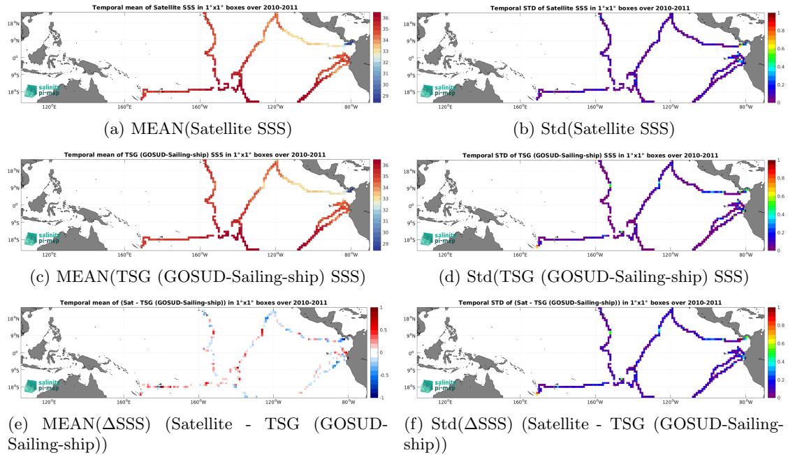
Figure 6: Temporal mean (left) and Std (right) of SSS from SMOS SSS L3 v8 - 9 Days (CATDS-CEC-LOCEAN) (top), TSG (GOSUD-Sailing-ship) (middle), and of \Delta SSS (Satellite - TSG (GOSUD-Sailing-ship)). Only match-up pairs are used to generate these maps.
