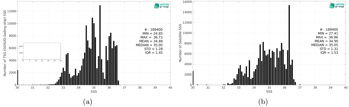
Figure 2: Histograms of SSS from TSG (GOSUD-Sailing-ship) (a) and SMOS SSS L3 v8 - 9 Days (CATDS-CEC-LOCEAN) (b) considering all match-up pairs per bins of 0.1 over the Tropical Pacific Ocean Pi-MEP region and for the full satellite product period.
