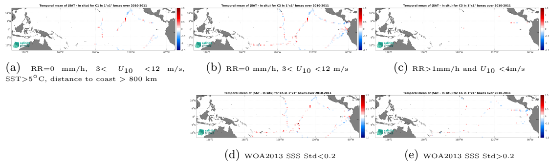
Figure 12: Temporal mean gridded over spatial boxes of size 1^{\circ}\times 1^{\circ} of \Delta SSS (SMOS SSS L3 v8 - 9 Days (CATDS-CEC-LOCEAN) - TSG (GOSUD-Sailing-ship)) for 5 different subdatasets corresponding to:RR=0 mm/h, 3 < U_{10} < 12 m/s, SST >5^{\circ}\text{C} , distance to coast > 800 km (a), RR=0 mm/h, 3 < U_{10} < 12 m/s (b), RR >1 mm/h and U_{10} < 4 m/s (c), WOA2013 SSS Std <0.2 (d), WOA2013 SSS Std >0.2 (e).
